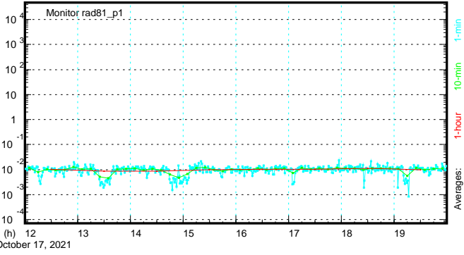
RM-81( \gamma ) (mrad/h) - Upstream of Forward Calorimeter
