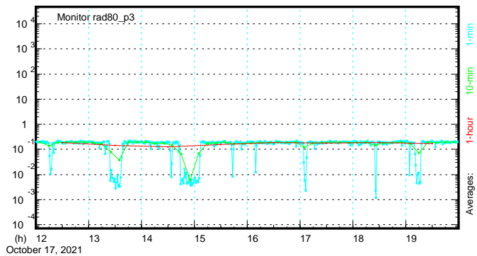
RM-80( \gamma ) (mrad/h) - Upstream of Solenoid magnet (BL)
