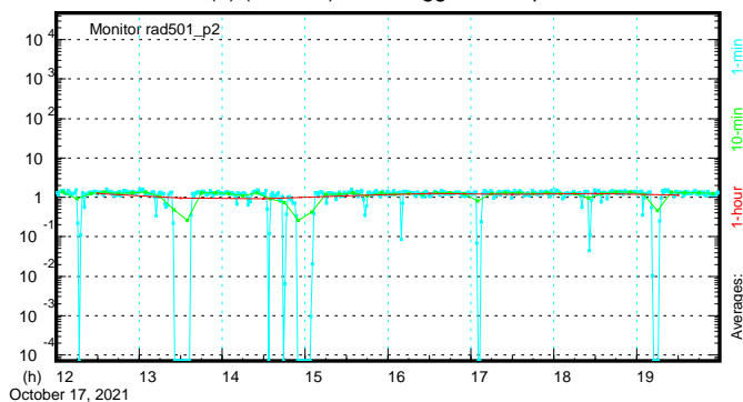
RM-501(n) (mrem/h) - XD Tagger Transport Tunnel
