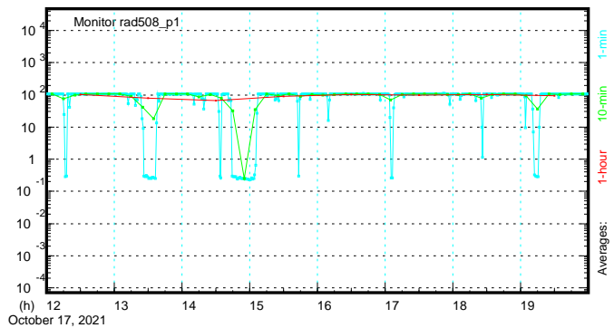
RM-508( \gamma ) (mrad/h) - XD Collimator Cave
