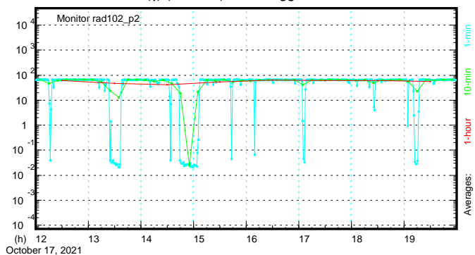
RM-102( \gamma ) (mrem/h) - XD Tagger Electr. Racks
