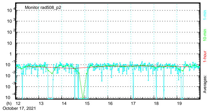
RM-508(n) (mrem/h) - XD Downstream Solenoid
