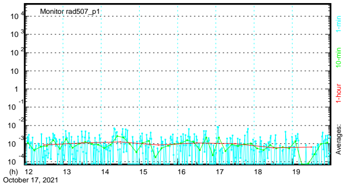
RM-507( \gamma ) (mrad/h) - XD Access Stairwell
