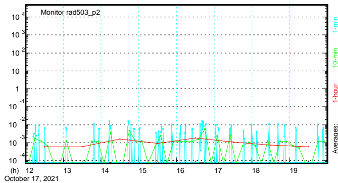
RM-503( \gamma ) (mrad/h) - XD Tagger Svce. Bldg.
