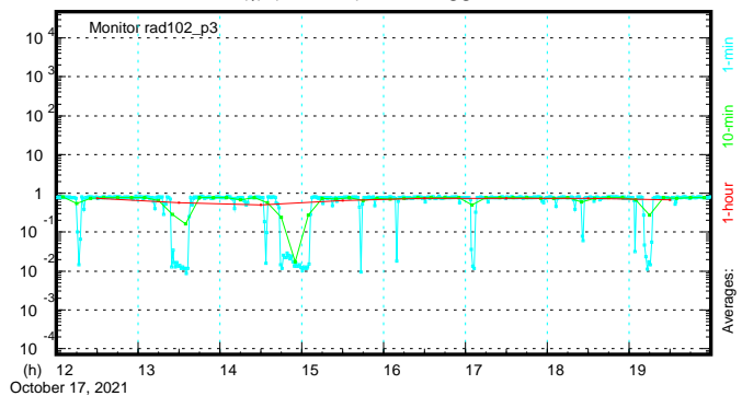
RM-102( \gamma ) (mrem/h) - XD Tagger Beam Line
