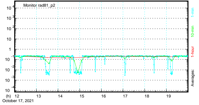
RM-81( \gamma ) (mrad/h) - Downstream of Forward Calorimeter (BL)
