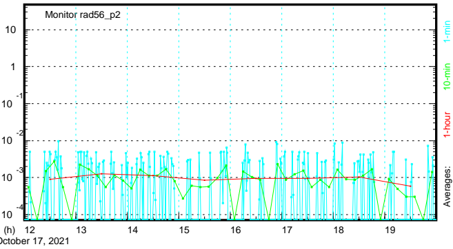
RM-56(n) (mrem/h) - Boundary Monitor RBM-8
