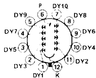
Figure 6 – Basing Diagram, Bottom View (For Temporary Base JEDEC No. B12-43)
