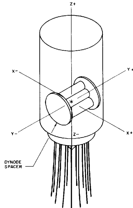
Figure 2 – Orthogonal Axes of Tube Used During Environmental Tests
