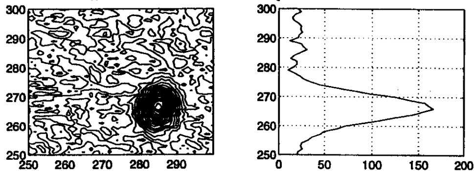
Figure 3. OTR profile and summed channels vs y (1 mm=8 ch) for 2.5 \mu\text{A} beam.
