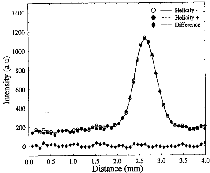
Figure 4. Helicity-correlated OTR beam profiles (summed channels vs y , 1 mm=16 ch) for 2.5 \mu\text{A} beam.
