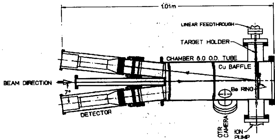
Figure 2. A schematic view of the Jefferson Lab 5 MeV Mott polarimeter.
