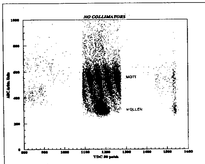
Figure 5. A plot of the pulse height versus the event time for one of the Møller electron detectors in time coincidence with the other electron detector, with the collimators fully open. Each scattering event is a dot on this plot. The pulse height is proportional to the detected electron energy. The incident electron beam had a 499 MHz time structure, so the beam bursts are 2 nsec apart, equal to 80 TDC channels. One can clearly see Møller scattered electrons in time coincidence with other Møller scattered electrons, and in accidental coincidence with Mott scattered electrons.
