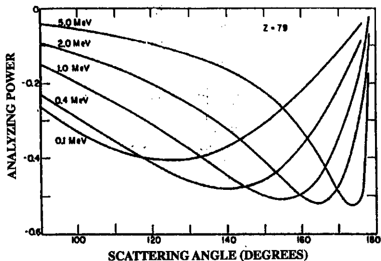
Figure 1. The Mott scattering analyzing power for gold as a function of scattering angle and electron energy, from J. Kessler, Rev. Mod. Phys. 41, 3 (1969).
