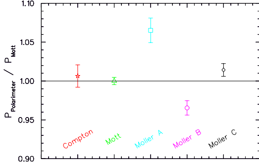
Figure 5: Relative analyzing power of the five electron beam polarimeters normalized to the Mott for comparison.
