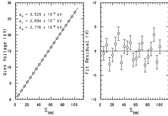
Figure 2: Differential Wien voltage with fit (left) and residuals (right) shown versus DAC setpoint ( S_{DAC} ).
