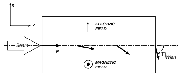
Figure 1: Diagram of Wien filter indicating the rotation of the beam polarization relative to the beam direction ( \eta_{Wien} ) in crossed magnetic and electric fields ( \beta = \frac{E}{B} ).
