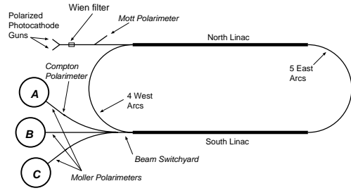
Figure 3: Schematic of the CEBAF 5-pass recirculating accelerator at JLab noting the Wien filter and five electron polarimeter locations.
