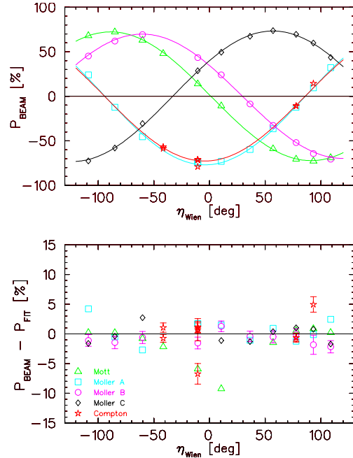
Figure 4: Polarimeter data and model fit ( upper plot ) with \lambda = 5.627^\circ/\text{kV} and fit residuals ( lower plot ). Uncertainties shown are only statistical.
