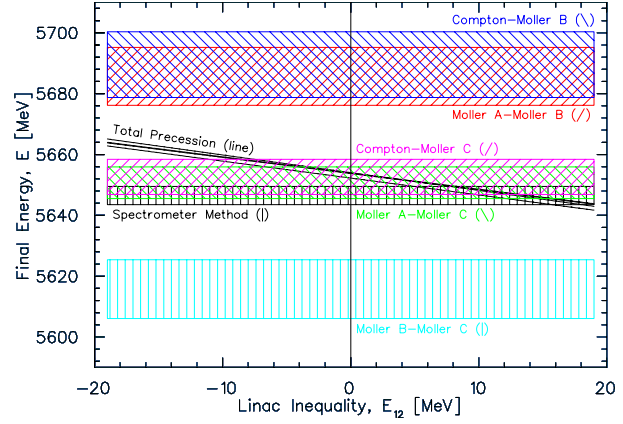
Figure 6: All energy results for |E_{12}| < 20 MeV.
