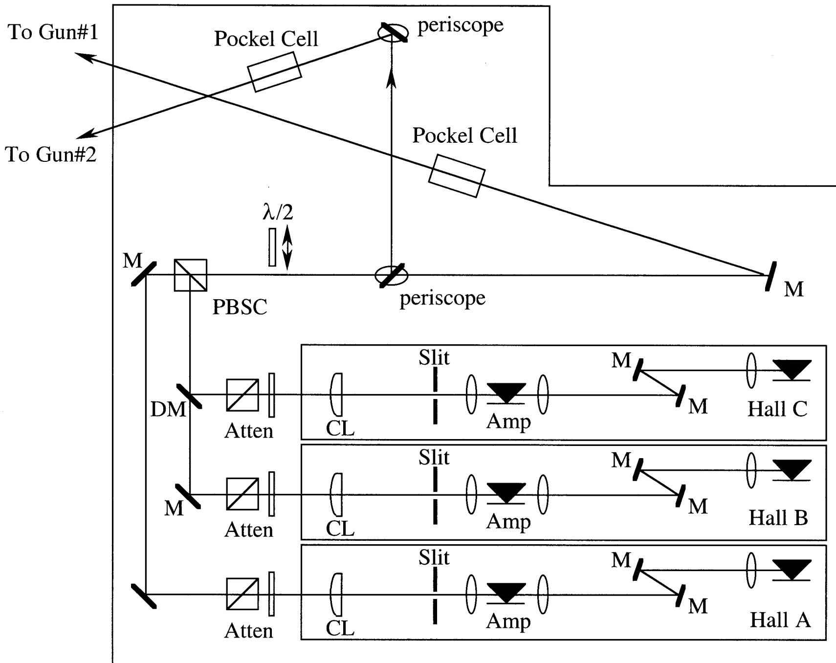
Present Diode Laser System for two Guns
