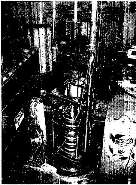
Figure 11. Preparation of an SNS cavity for test in the vertical test area (VTA).
