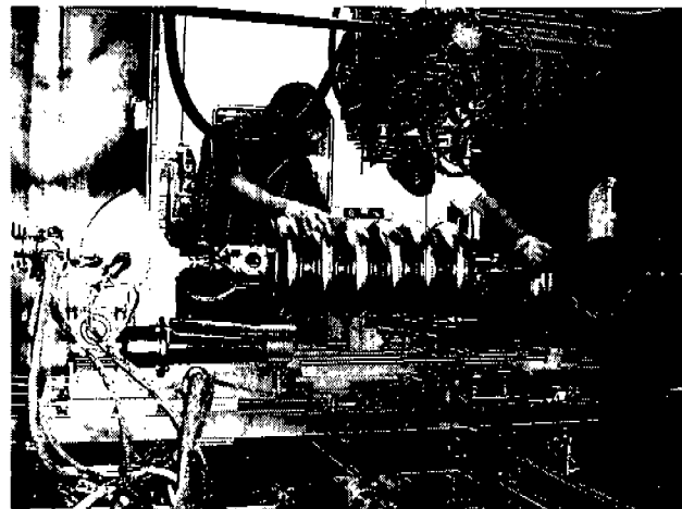
Figure 10. E-beam an SNS prototype cavity.
