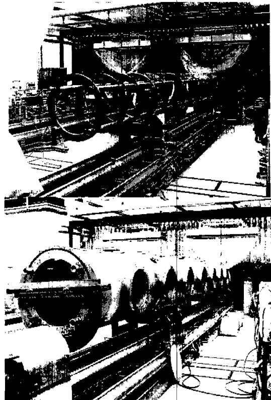
Figure 8. Upgrade cryomodule space frame and vacuum vessel.
