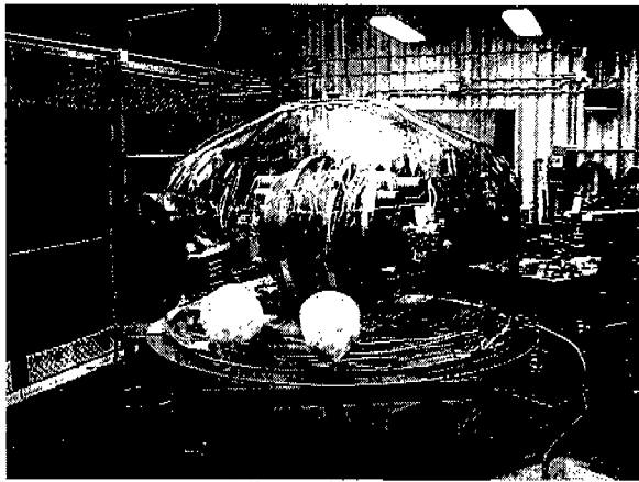
Figure 12. TIG welding of an SNS prototype cavity helium vessel.
