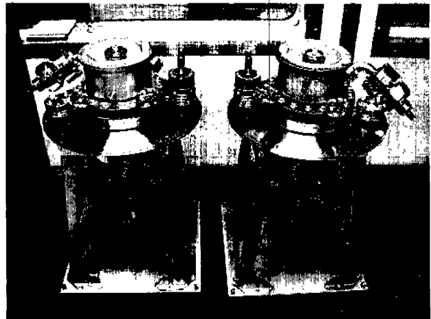
Figure 15. First SNS prototype input couplers.
