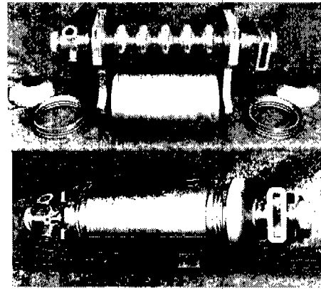
Figure 6. CEBAF Mk II upgrade cavity
