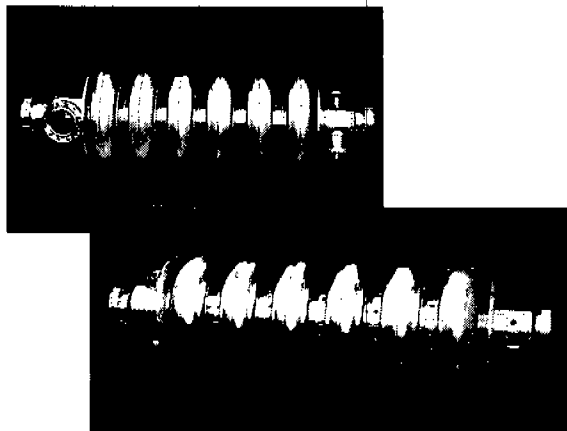
Figure 5. SNS prototype \beta=0.61 and 0.81 cavities.
