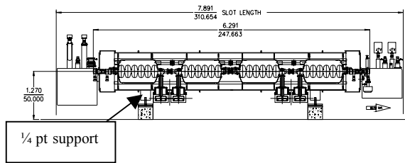
Figure 3, High \beta Cryomodule
