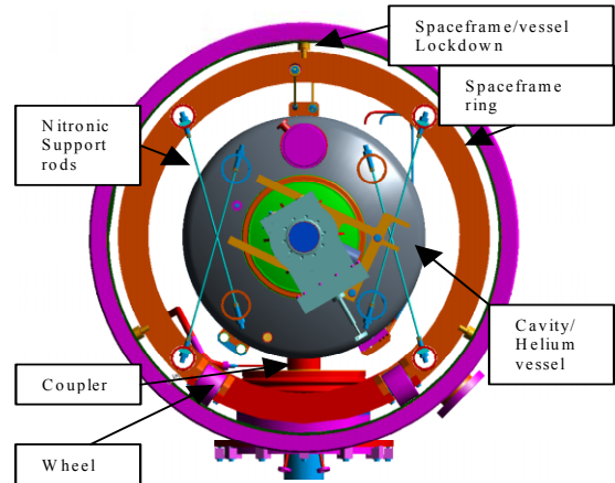
Figure 1 Medium \beta Cryomodule end view
