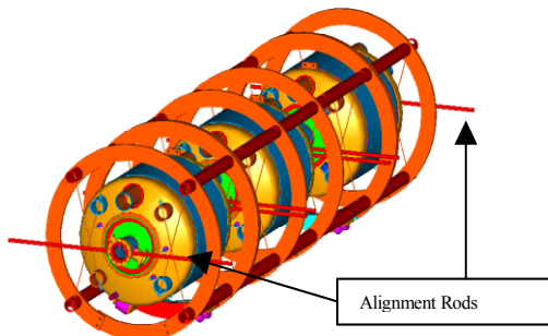
Figure 4 Cavity String Alignment
