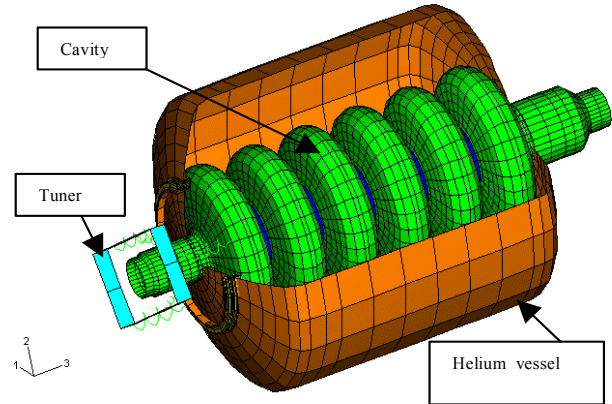
Figure 5: Medium \beta He vessel assembly FE model
