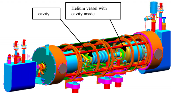
Figure 2 Medium \beta Cryomodule cutaway
