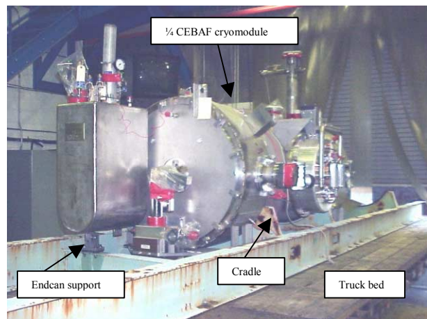
Figure 6 CEBAF \frac{1}{4} Cryomodule on air ride trailer
