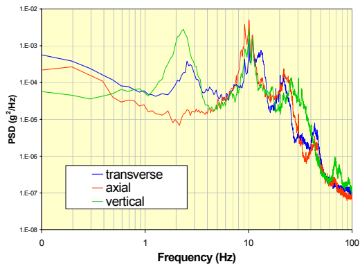
Figure 7 Road Test Vibration PSD of the Beamline
