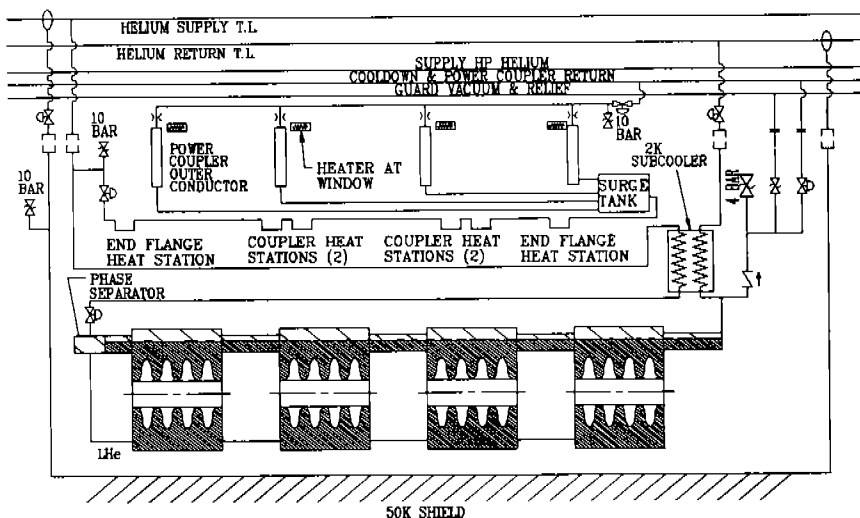
FIGURE 1. The High Beta Cryomodule Flow Schematic.
