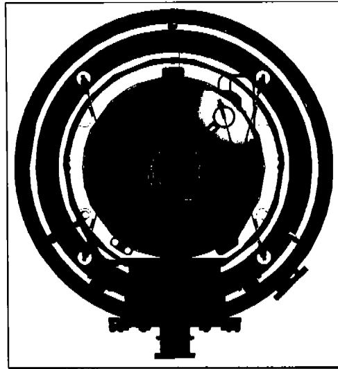
FIGURE 2. Nitronic-50™ Support Rods Attach the Helium Vessel Assembly to the Space Frame.
