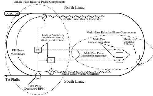
Figure 2: First-pass system (left-hand ellipse) and the multi-pass extension (right-hand ellipse) for measuring relative phase of beam and RF. Independent phase modulation signals are generated for the two linacs. The pickups for the multi-pass system are referenced to those remote signals and require no additional perturbation of the beam.
