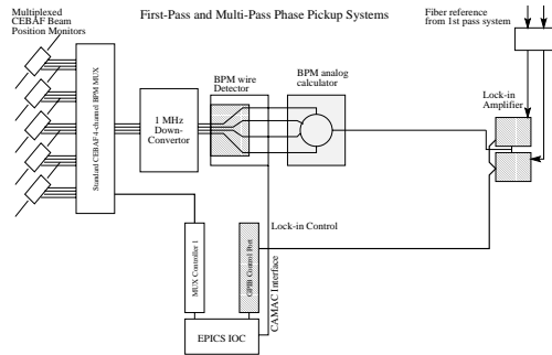
Figure 3: BPM and signal processing schematic for the recirculated beam.
