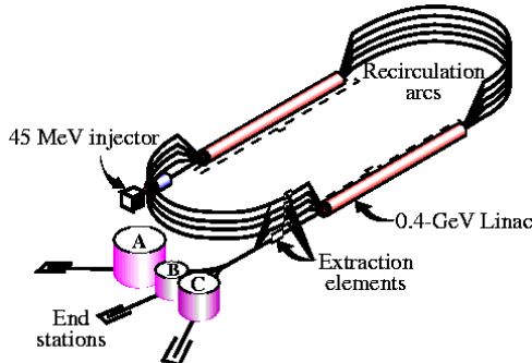
Figure 1: Layout of CEBAF Accelerator. The North Linac is at the upper left, immediately following the injector. The diagnostic reported here is about 80% of the way clockwise around recirculation arcs at the top right.
