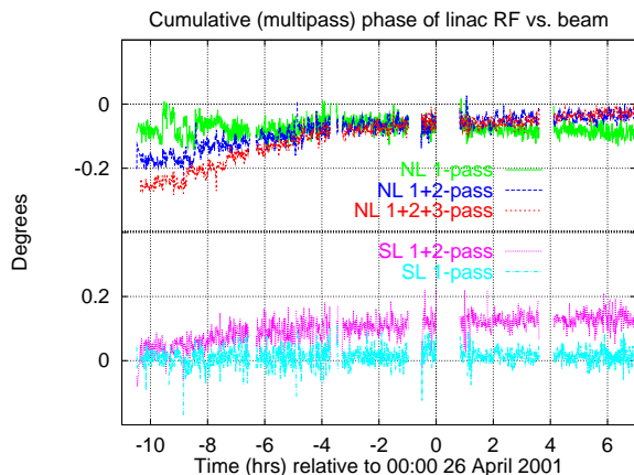
Figure 4: Example data for 100 \mu A of beam delivered on third pass to an experiment in Hall A. Gaps in the plots are during times when beam was interrupted. The traces appear from top to bottom as in the legend. No path length correction was attempted during this time span.
