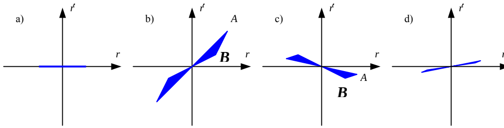
Fig. 4.3.8-1. Transverse phase space plots schematically showing the emittance compensation technique (Carlsten, 1989). a) initial phase space with small emittance at the gun; b) phase space after transport to the solenoid lens, showing the growth of the projected emittance due to the different space charge defocusing force at the bunch center (A) and the tails (B); c) the phase space distribution has been rotated by an external focusing kick; d) phase space after a drift behind the lens, showing the projected emittance reduction due to the different expansion rates of points A and B.
