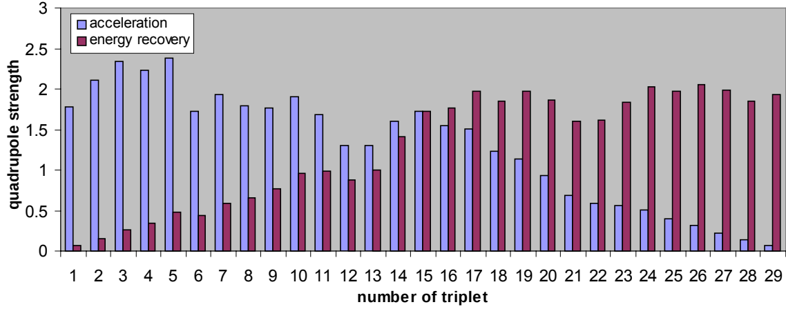
Fig. 3.1.4-3. Strength |k| in [\text{m}^{-2}] of the middle quadrupole in a triplet along the SRF structure corresponding to Fig. 3.1.4-5.
