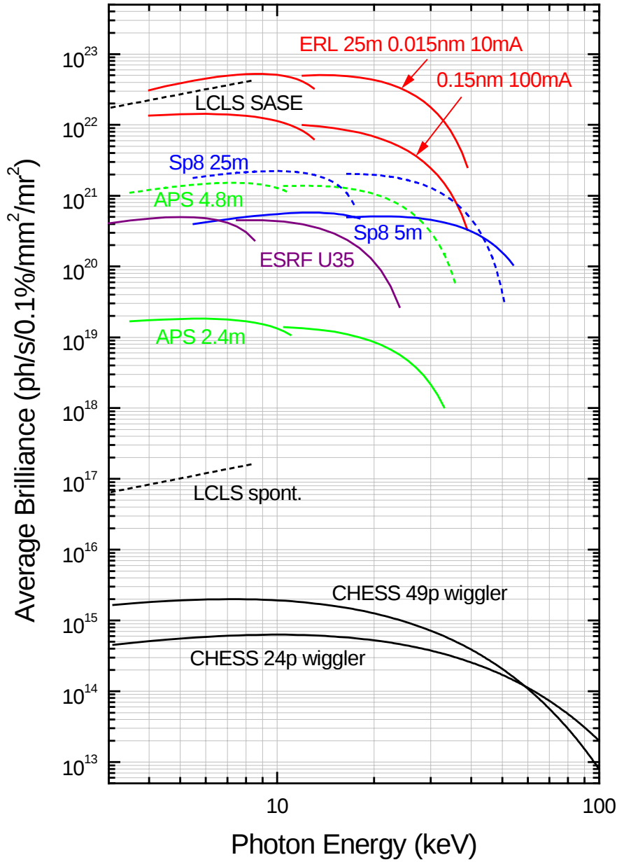
Figure 2.2-1: Comparison of calculated average spectral brilliance of the various sources. The parameters used for undulator sources are listed in Table 2.2-1. The CHESS wiggler sources assume 5.3 GeV 300 mA operation and a FWHM source size of d_x = 5.5 mm and d_y = 0.9 mm for the 24-pole wiggler at F-line and d_x = 3.3 mm and d_y = 0.85 mm for the 49-pole wiggler at A/G-line.
