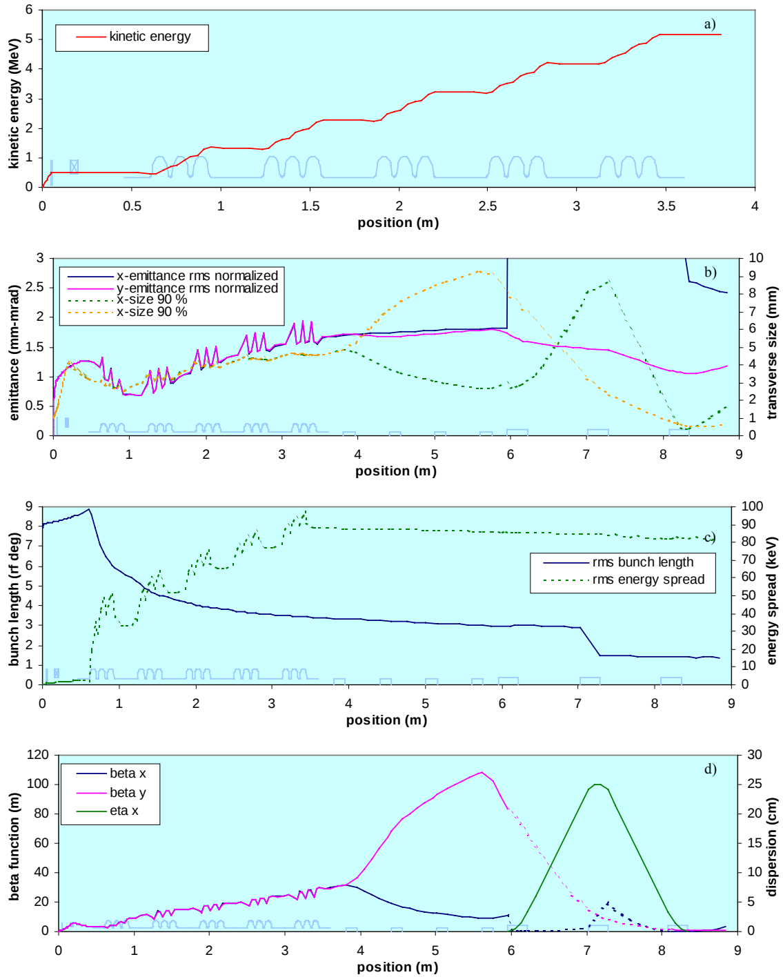
Fig. 4.3.8-9. Various parameters vs. longitudinal position in the injector with 5 three-cell SRF capture cavities (compressed by a factor of 6). Locations of cathode, anode, solenoid, cavities, quadrupoles and dipoles are shown (see Table 4.3.8-2). a) kinetic energy; b) transverse emittance and bunch size (the envelope includes 90 % of the particles); c) bunch length and energy spread; d) betatron and dispersion functions (dashed lines show betatron functions in the achromat section).
