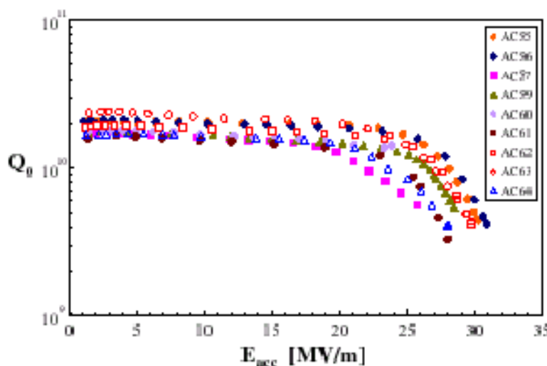
Figure 5.2.3.1-1: TTF cavity results (TESLA 2001).
