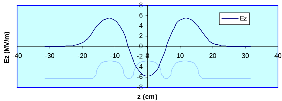
Fig. 4.3.8-7. Axial electric field profile in a 3-cell cavity.
