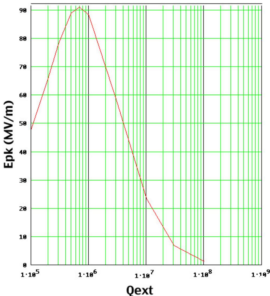
Fig. 5.2.3.1-5. Peak electric field reachable with 1.5 MW of RF power and pulse length of 250 \mu\text{s} as a function of the setting of the input coupler Q_{\text{ext}} . HPP experience shows that after reaching 90 MV/m peak field, a cavity will operate free of field emission at E_{\text{acc}} = 22.5 MV/m.
