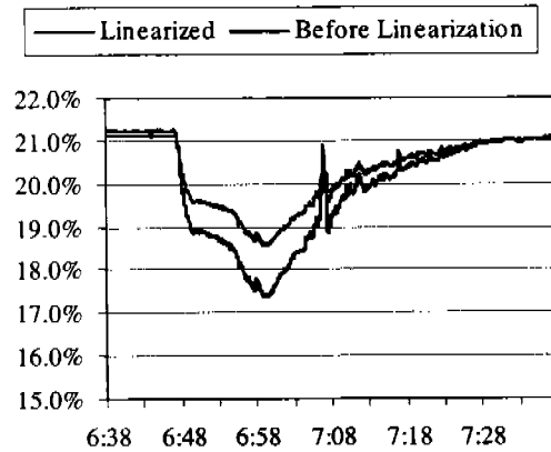
Figure 7. Sample spill test data (OM13) relinearized using (6).
