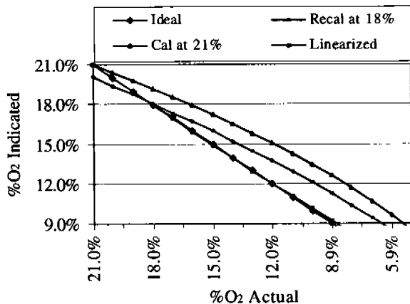
Figure 6. Relinearization of sensor calibrated at 18% oxygen in air/helium.
