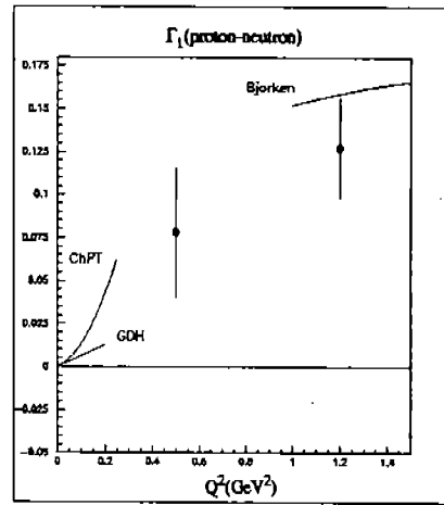
Figure 1. First moment of the spin structure function g_1(x, Q^2) for the proton and neutron (left), and for the proton-neutron difference (right). The curves above Q^2 = 1 \text{ GeV}^2 are pQCD evolutions of the measured \Gamma_1 for proton and neutron, and the pQCD evolution for the Bjorken sum rule, respectively. The straight lines near Q^2 = 0 are the slope given by the GDH sum rule. The curves at small Q^2 represent the NLO HBChPT results.
