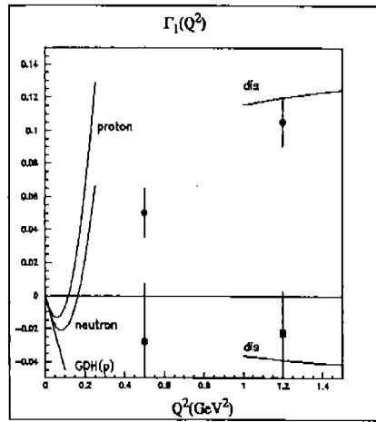
Figure 1. First moment of the spin structure function g_1(x, Q^2) for the proton and neutron (left), and for the proton-neutron difference (right). The curves above Q^2 = 1 \text{ GeV}^2 are pQCD evolutions of the measured \Gamma_1 for proton and neutron, and the pQCD evolution for the Bjorken sum rule, respectively. The straight lines near Q^2 = 0 are the slope given by the GDH sum rule. The curves at small Q^2 represent the NLO HBChPT results.
