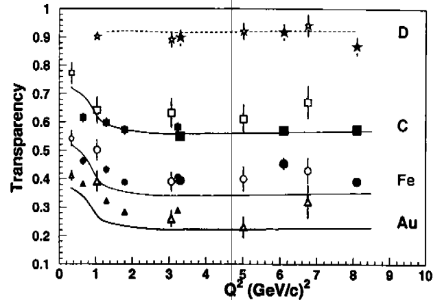
FIG. 3. Transparency for (e,e'p) quasielastic scattering from D (stars), C (squares), Fe (circles), and Au (triangles). Data from the present work are the large solid stars, squares, and circles, respectively. Previous JLab data (small solid squares, circles, and triangles) are from Ref. [16]. Previous SLAC data (large open symbols) are from Ref. [8,9]. Previous Bates data (small open symbols) at the lowest Q^2 on C, Ni, and Ta targets, respectively, are from Ref. [25]. The errors shown include statistical and systematic ( \pm 2.3\% ) uncertainties, but do not include model-dependent systematic uncertainties on the simulations. The solid curves shown from 0.2 < Q^2 < 8.5 \text{ (GeV/c)}^2 are Glauber calculations from Ref. [26]. In the case of D, the dashed curve is a Glauber calculation from Ref. [27].
