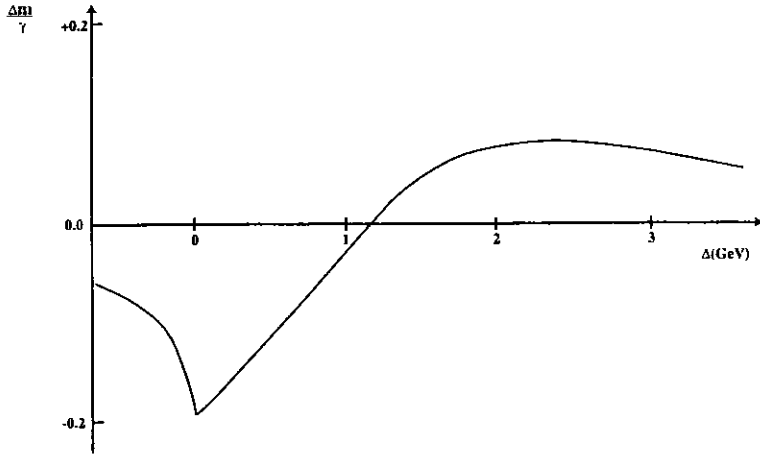
Fig. 2: a typical S -wave mass shift and its dependence on \Delta \equiv m^{\text{valence}} - m^{\text{threshold}} , shown is \Delta m/\gamma for K_0^* \rightarrow K\pi \rightarrow K_0^* for the simple width function \Gamma = \gamma q e^{-q^2} with q in GeV.
