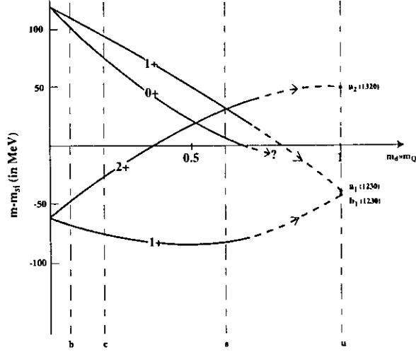
Fig. 3: The m_Q -dependence of the P -wave spectra (solid curves). Vertical lines show the values of m_d/m_Q corresponding to each of Q = u, s, c and b . The dashed curves illustrate possible connections to the observed (and unobserved) u\bar{d} states.
