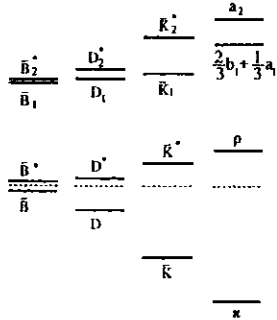
Fig. 1: the evolution of Q\bar{d} spectra from Q = b to Q = u ; \bar{B}_2^* and B_1 , which are not yet separately identified, are shown here with their measured center-of-gravity and predicted splitting.
