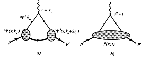
FIG. 2. a) Structure of the effective two-body contribution to form factor in the light cone formalism. b) Form factor as an x -integral of nonforward parton densities.
