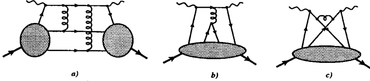
FIG. 6. Configurations involving double and single gluon exchange.
