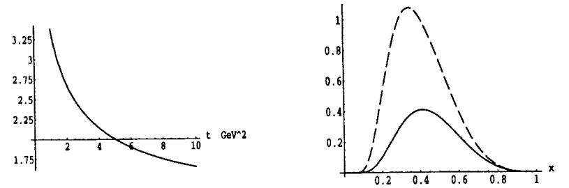
FIG. 7. a) Ratio R_1^a(t)/F_1^a(t) ; b) Functions \mathcal{F}^a(x; t) (solid line) and \mathcal{F}^a(x; t)/x (dashed line) at t = -2.5 \text{ GeV}^2 .
