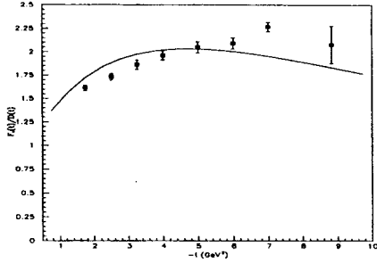
FIG. 3. Ratio F_1^p(t)/D(t) of the F_1^p(t) form factor to the dipole fit D(t) = 1/(1 - t/0.71 \text{ GeV}^2)^2 . Curve is based on Eqs.(16)-(18) and experimental data are taken from ref.[18].
