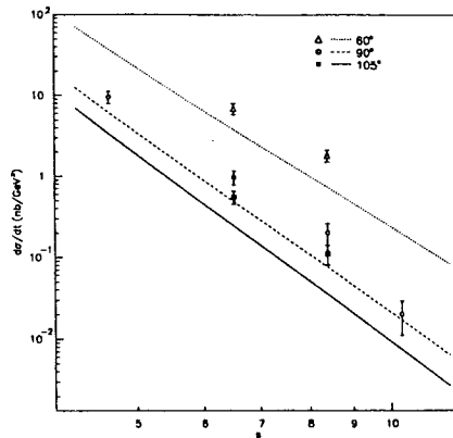
FIG. 10. s -dependence of the combination s^0 d\sigma/dt for \theta = 60^\circ (dotted line), \theta = 90^\circ (dashed line) and \theta = 105^\circ (solid line).
