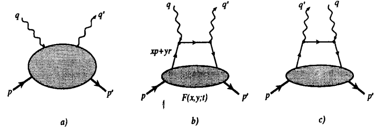
FIG. 1. a) General Compton amplitude; b) s -channel handbag diagram; c) u -channel handbag diagram.
