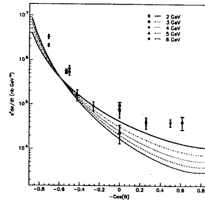
FIG. 9. Angular dependence of the combination s^6(d\sigma/dt) .
