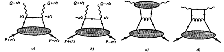
FIG. 5. Terms having O(s^0) behavior for large s .
