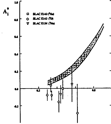
Figure 1(b): Data [4] on A_1^n and the prediction (shaded band) of the model described in the text; the SU(6) prediction is 0.
