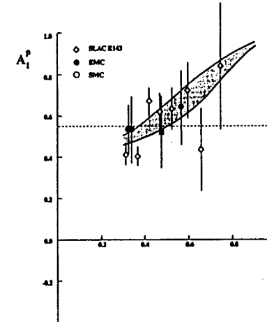
Figure 1(a): Data [4] on A_1^p and the prediction (shaded band) of the model described in the text; the SU(6) prediction is \frac{5}{9} (dotted line).
