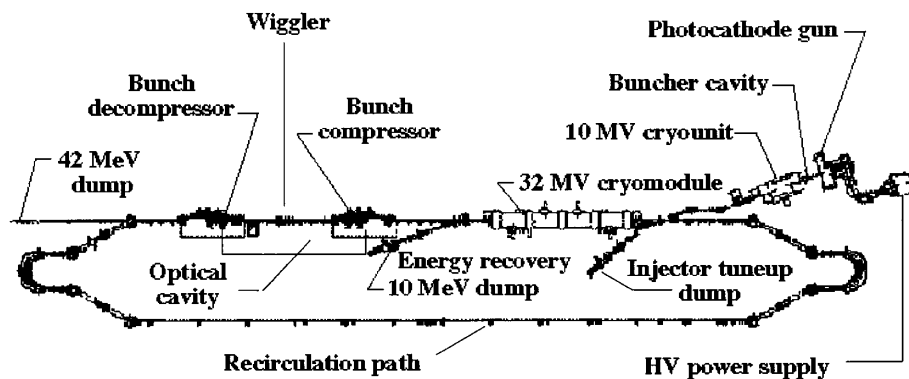
FIG. 1. Schematic of IR Demo; dimensions of the recirculation loop are roughly 49 \text{ m} \times 6 \text{ m} .
