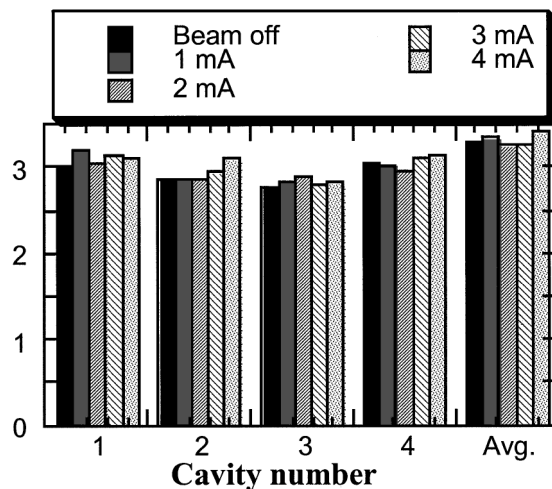
FIG. 2. Cryomodule rf power in watts versus recirculated current while lasing. The first four of eight cavities and the average of all eight cavities are shown. Variations in power are comparable to fluctuations due to microphonics.
