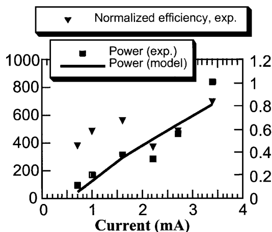
FIG. 3. Experimental power at 4.9 \mu\text{m} and product of the efficiency and 4N_W compared to theoretical power predictions. The power and efficiency were measured 28% from zero detuning to provide a comparison to models [17] and most stable operation. Current was changed by varying pulse charge at a fixed frequency of 37.4 MHz with no change in the mirror out-coupling.
