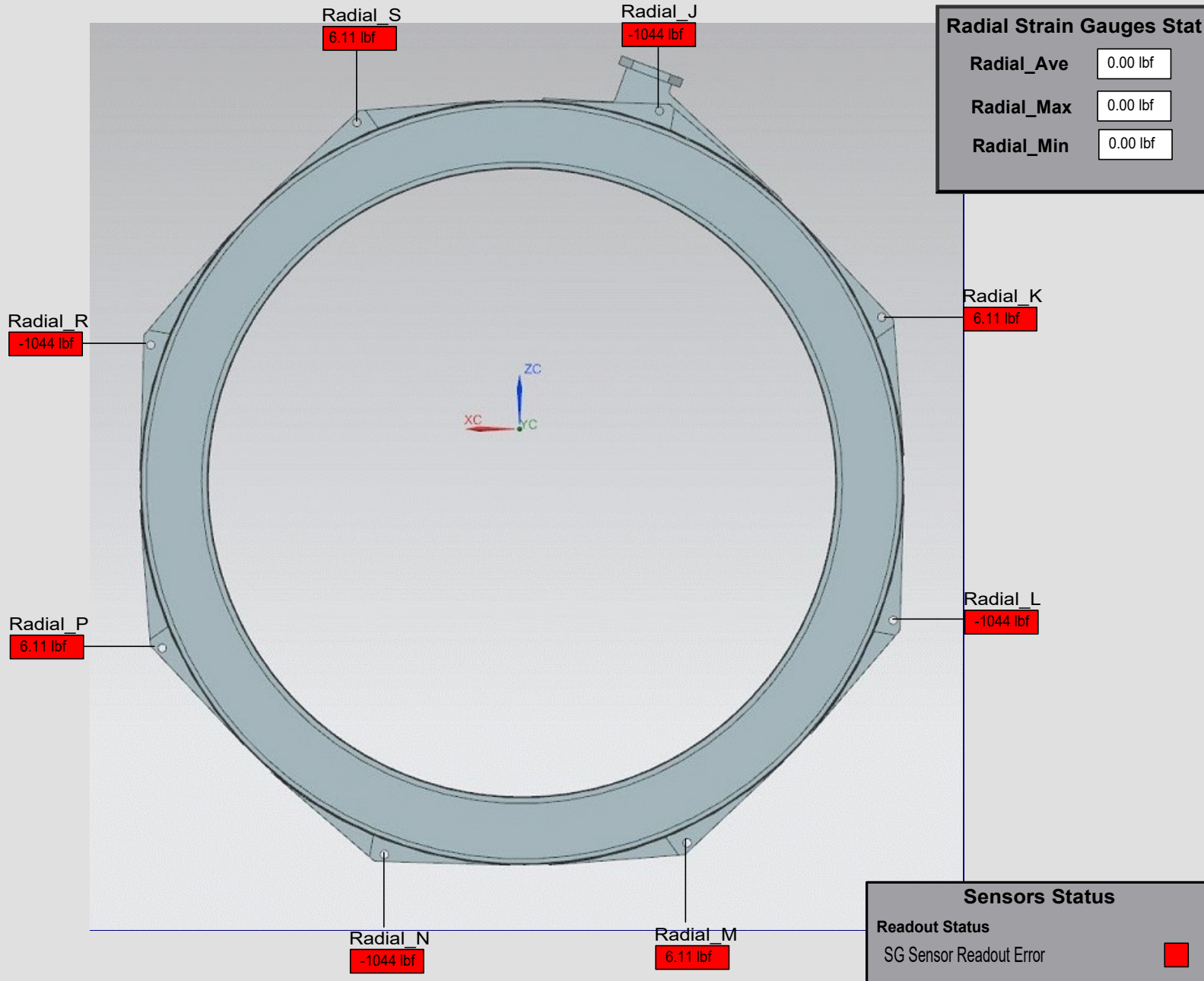
SoLID Magnet Downstream View
