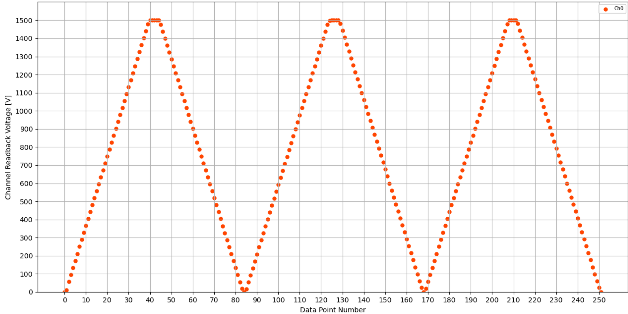
Voltage Ramp Test (Python) Bd #128, Slot #1, Ch #0
