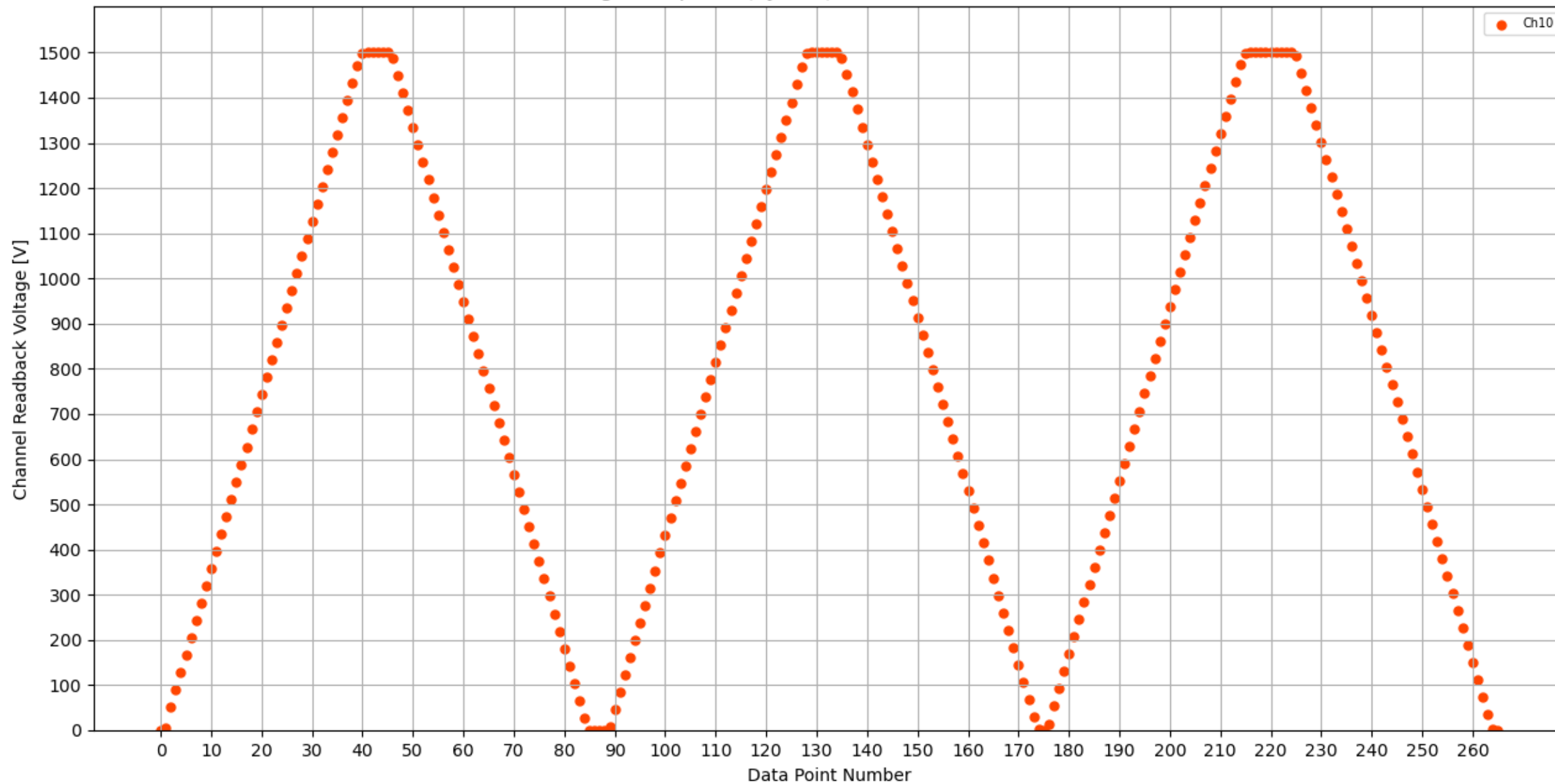
Voltage Ramp Test (Python) Bd #128, Slot #1, Ch #10
