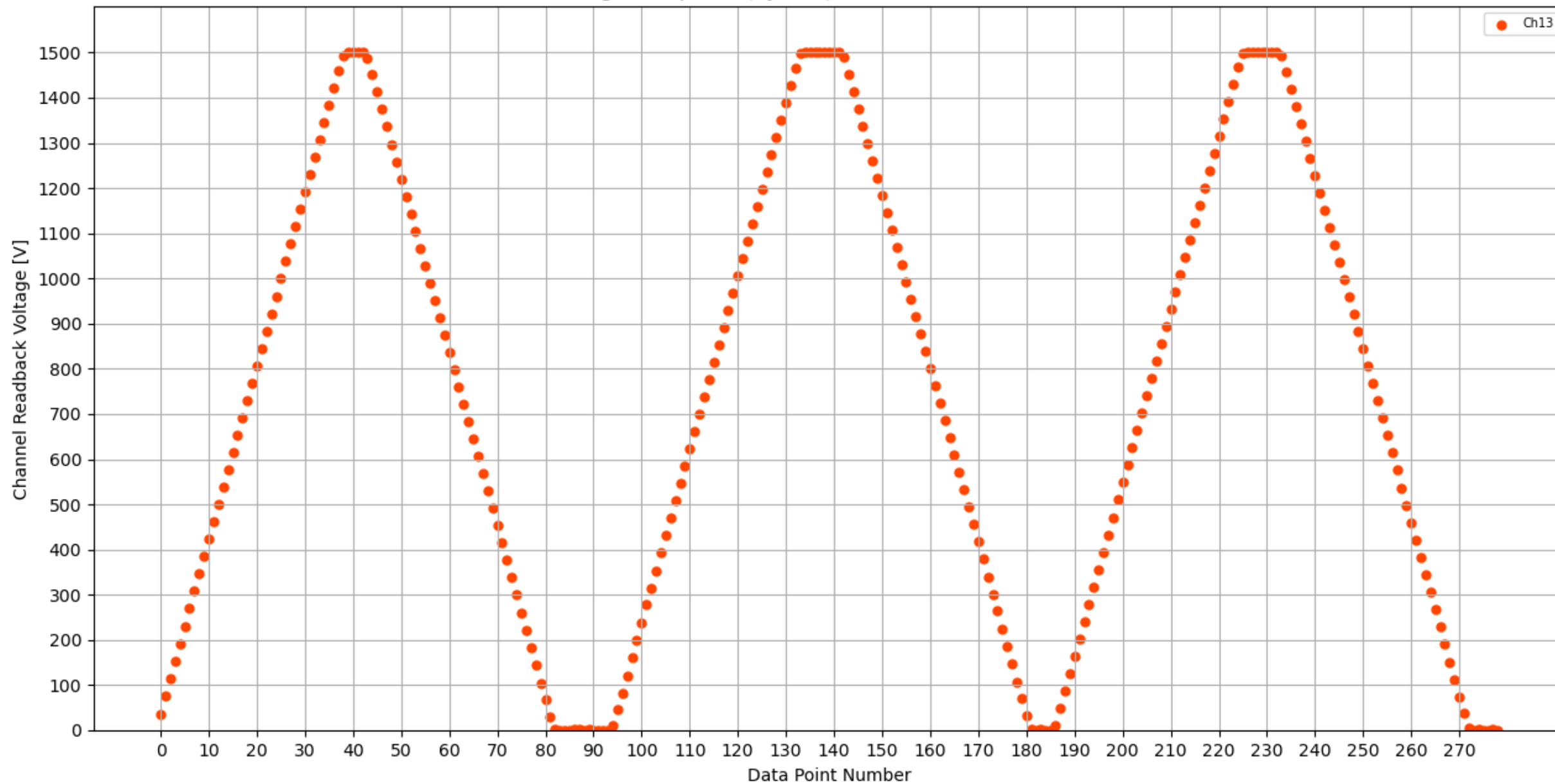
Voltage Ramp Test (Python) Bd #128, Slot #1, Ch #13
