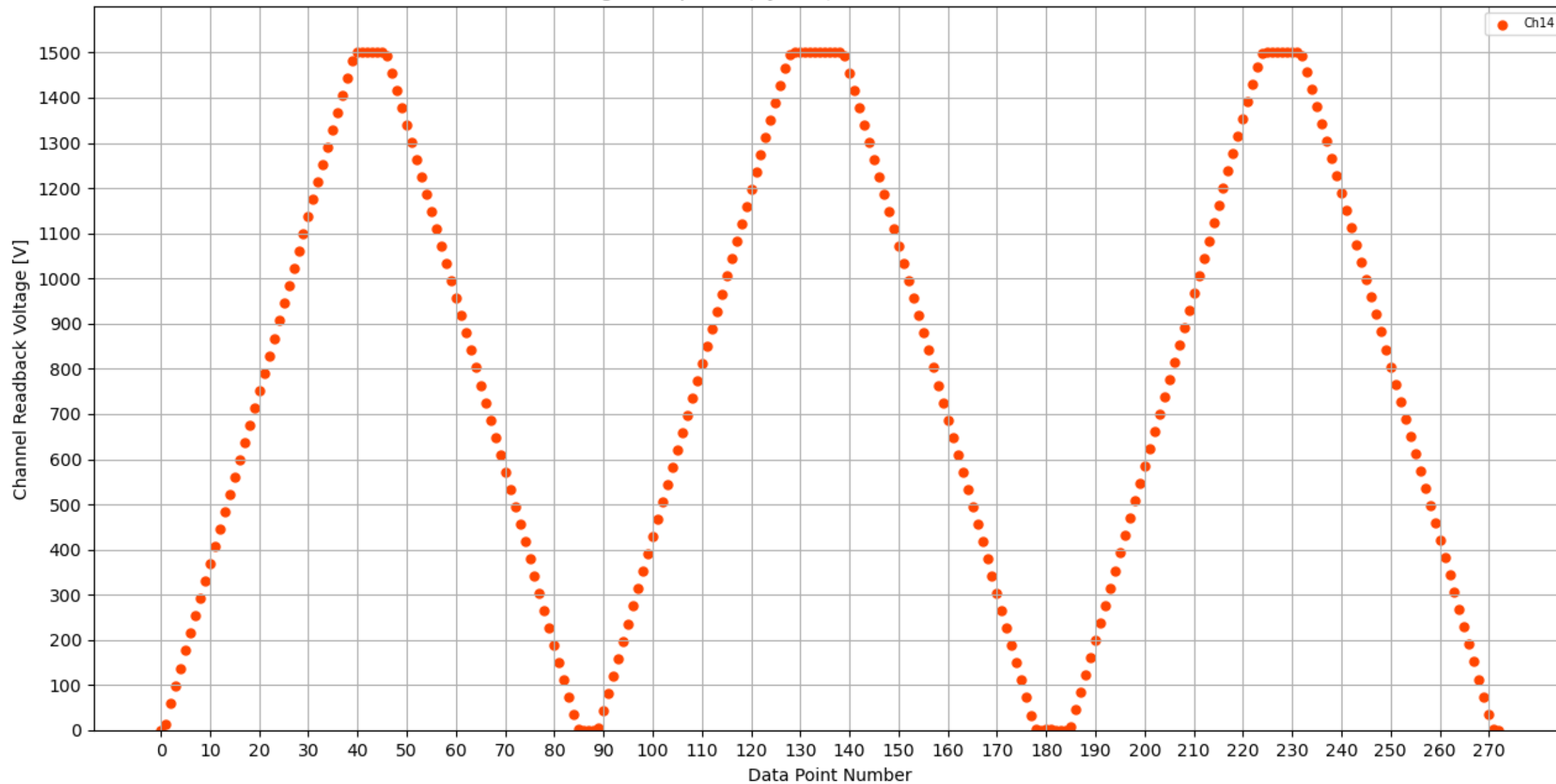
Voltage Ramp Test (Python) Bd #128, Slot #1, Ch #14
