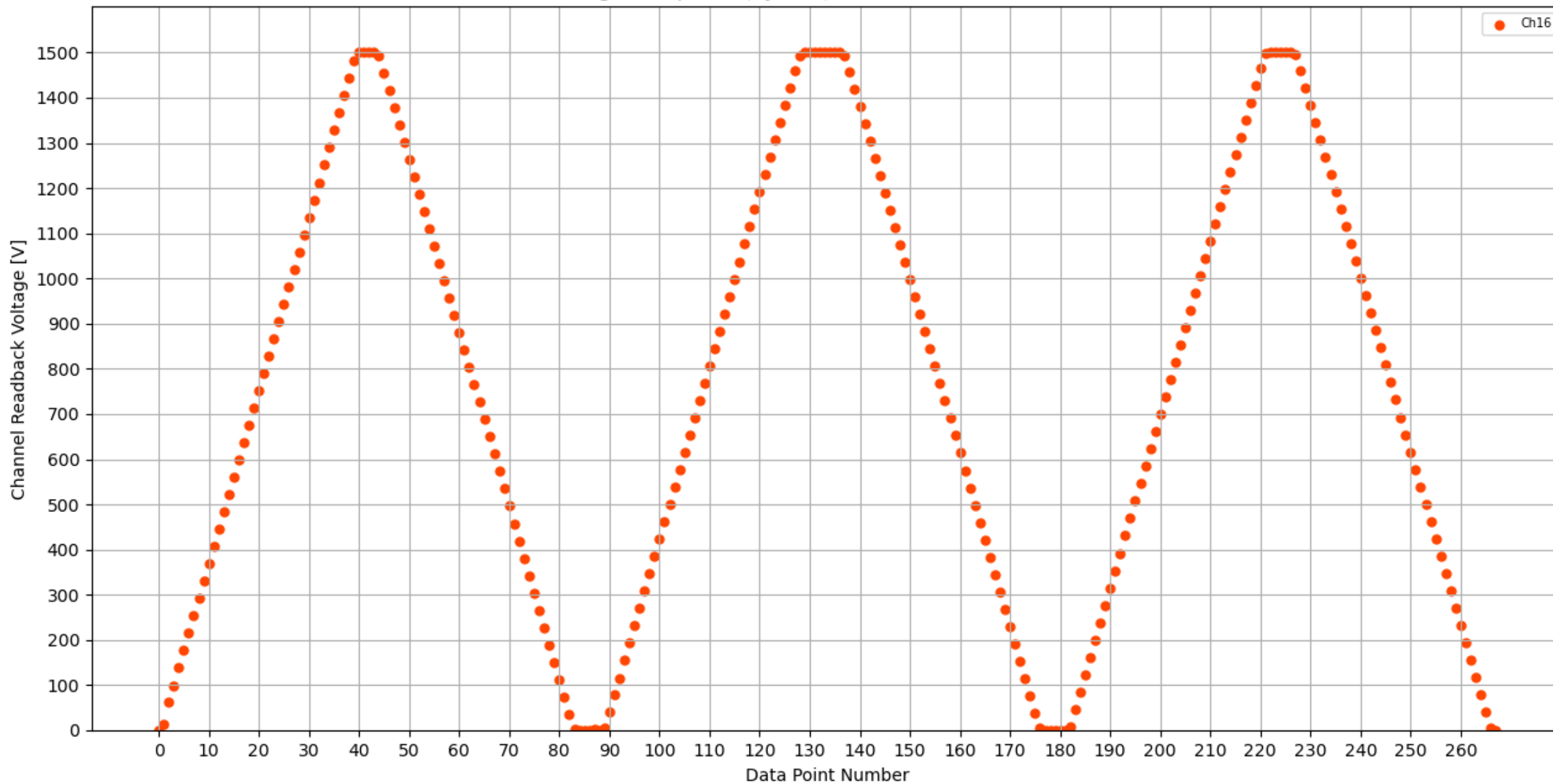
Voltage Ramp Test (Python) Bd #128, Slot #1, Ch #16
