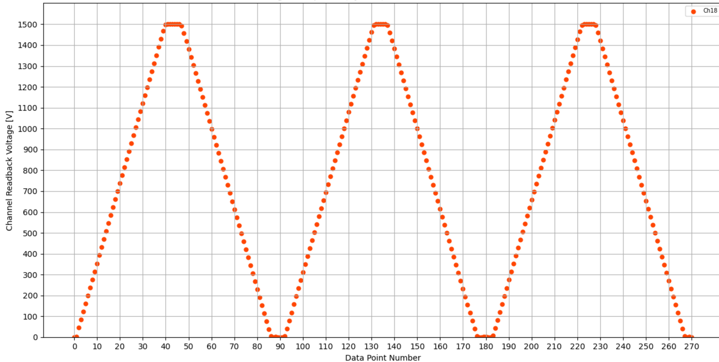
Voltage Ramp Test (Python) Bd #128, Slot #1, Ch #18
