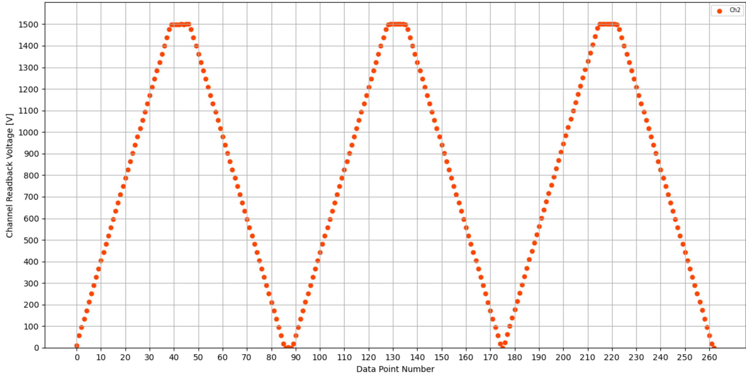
Voltage Ramp Test (Python) Bd #128, Slot #1, Ch #2
