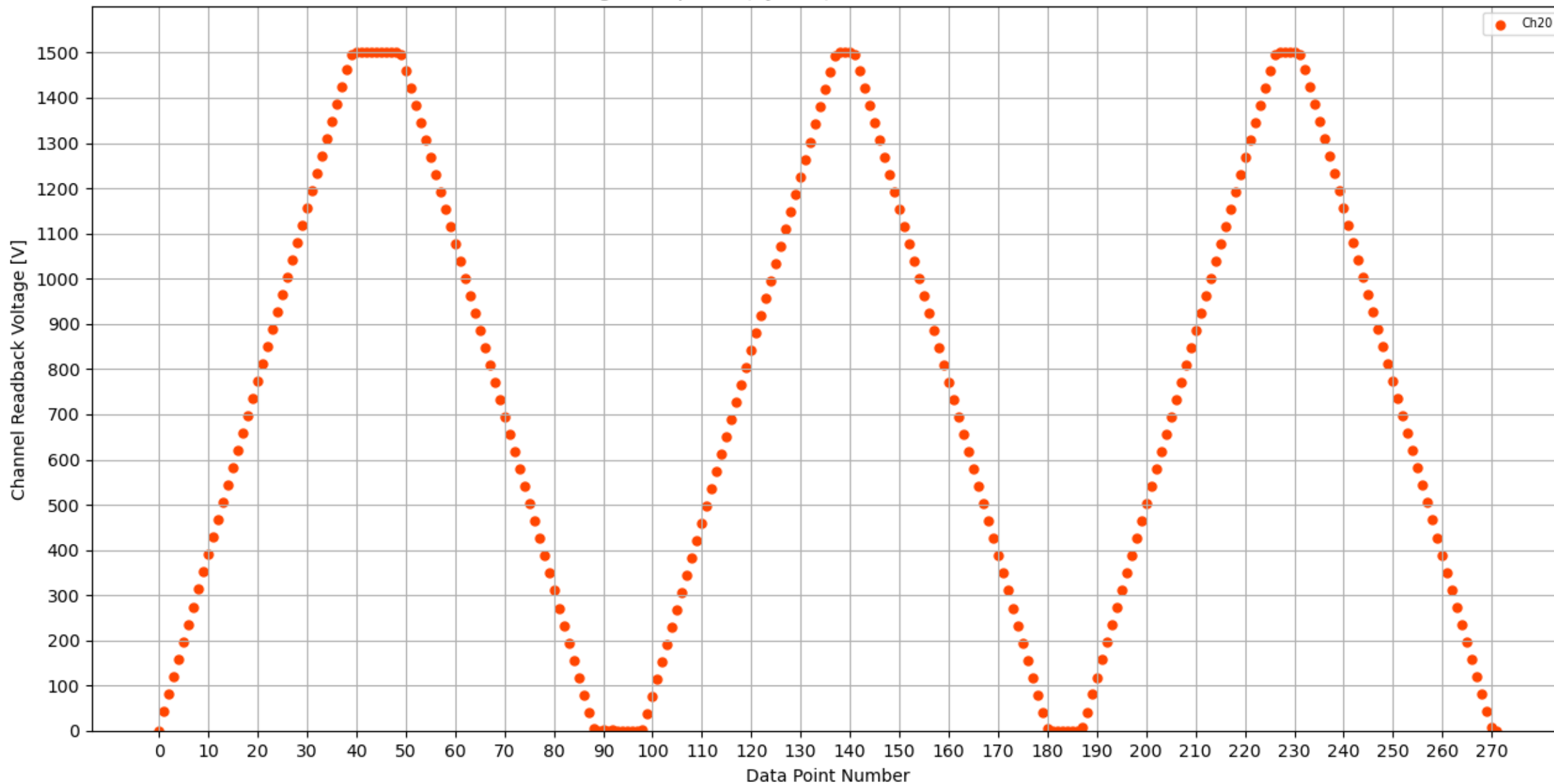
Voltage Ramp Test (Python) Bd #128, Slot #1, Ch #20
