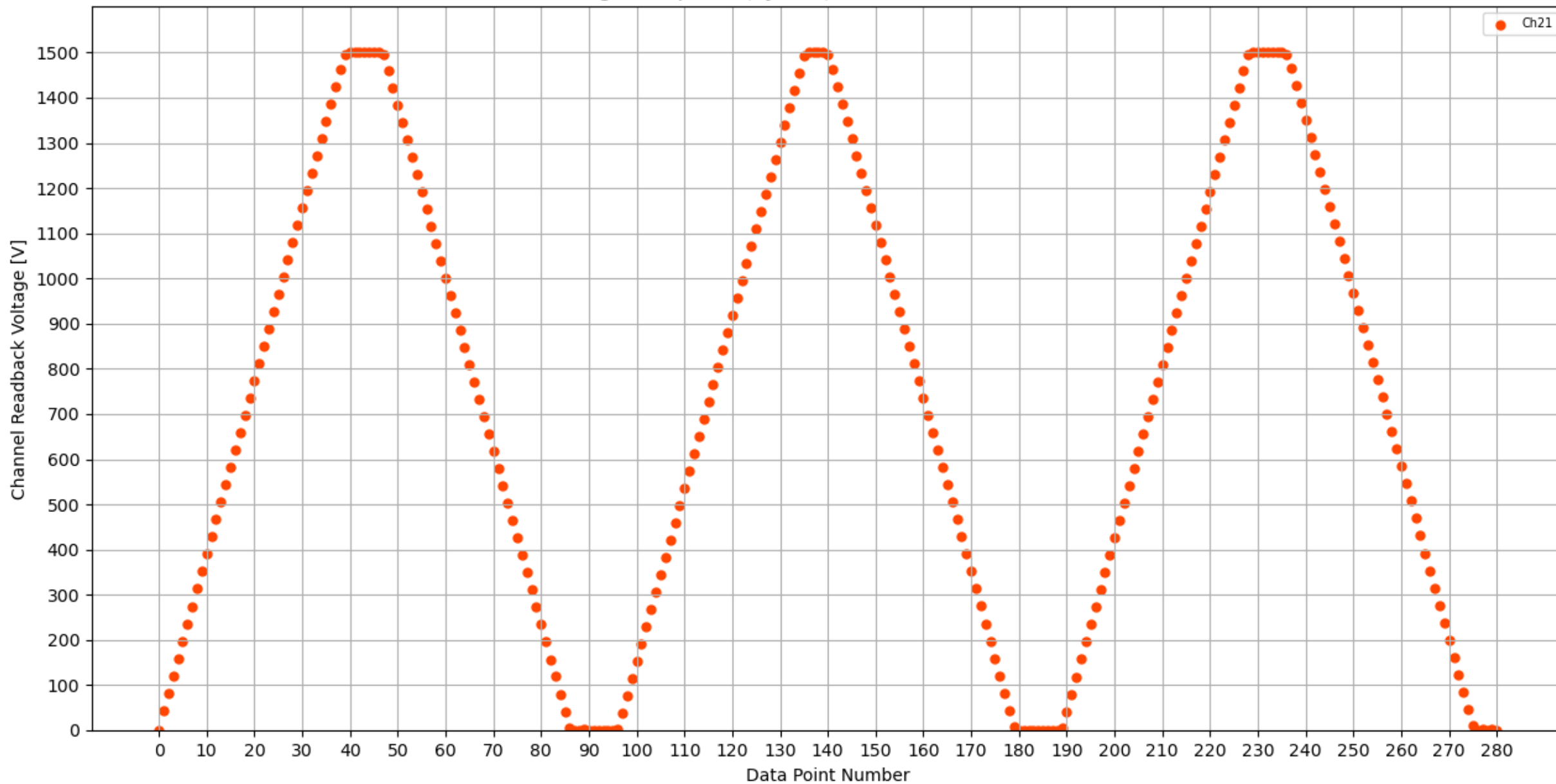
Voltage Ramp Test (Python) Bd #128, Slot #1, Ch #21
