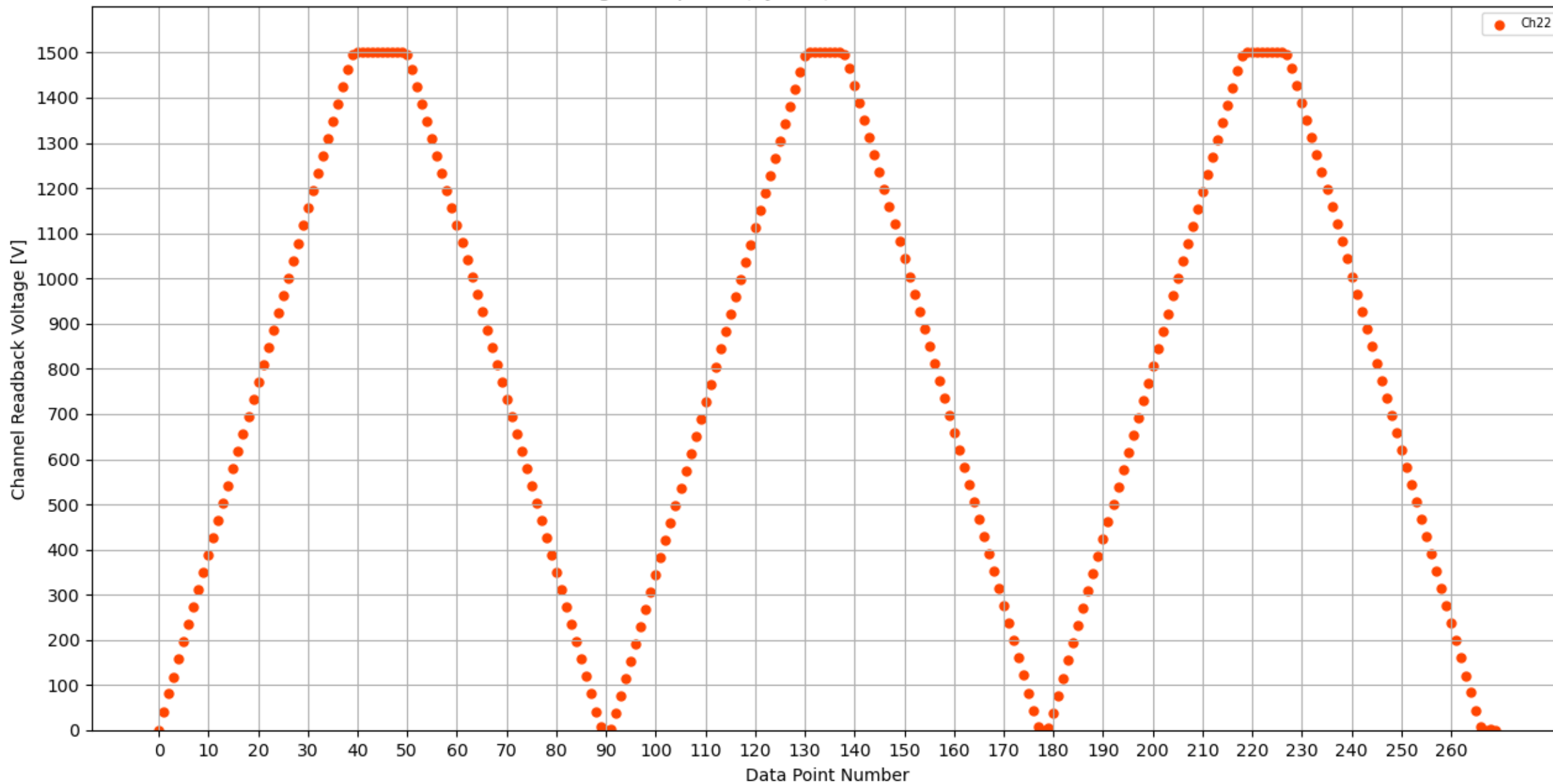
Voltage Ramp Test (Python) Bd #128, Slot #1, Ch #22
