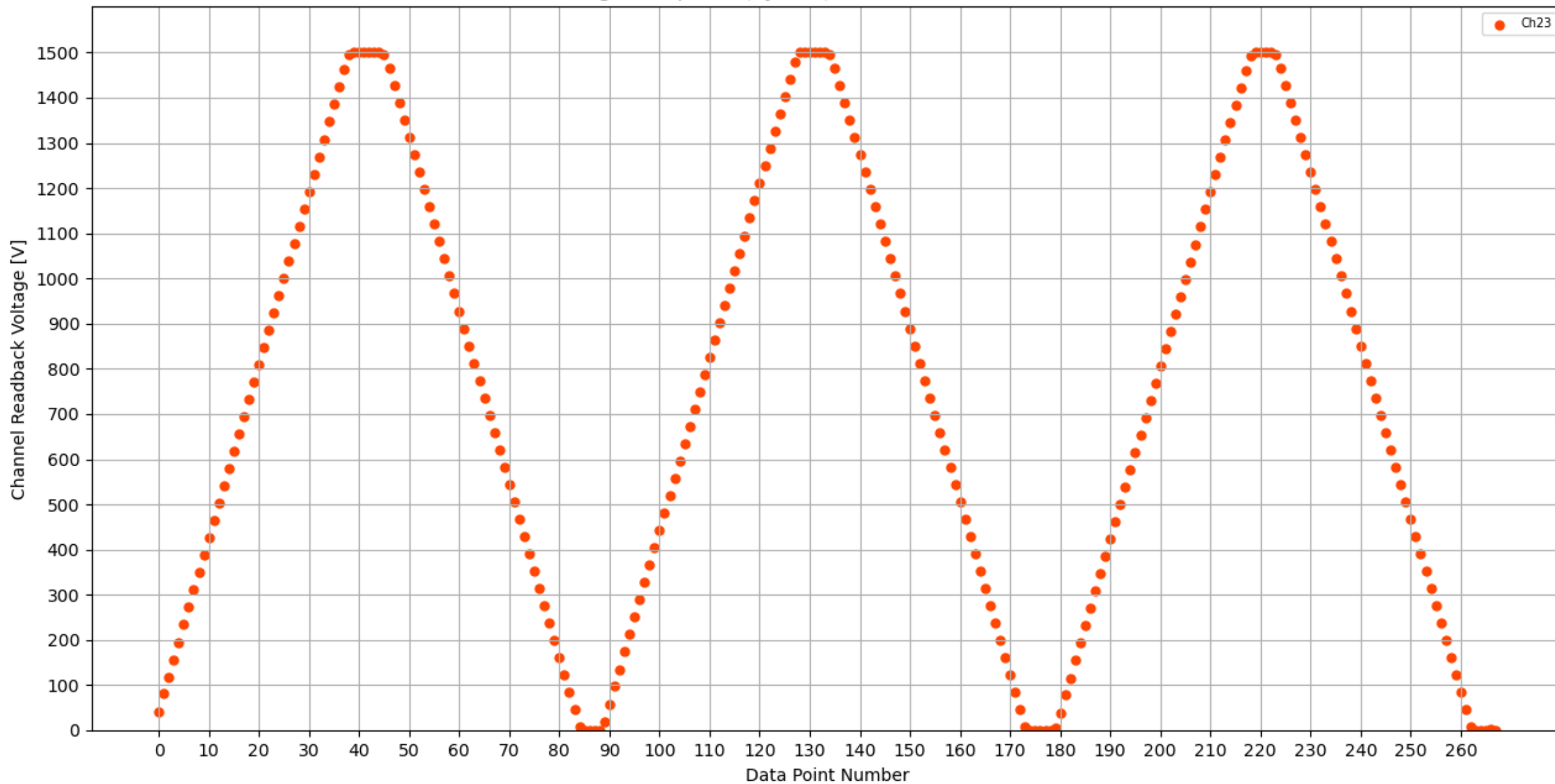
Voltage Ramp Test (Python) Bd #128, Slot #1, Ch #23
