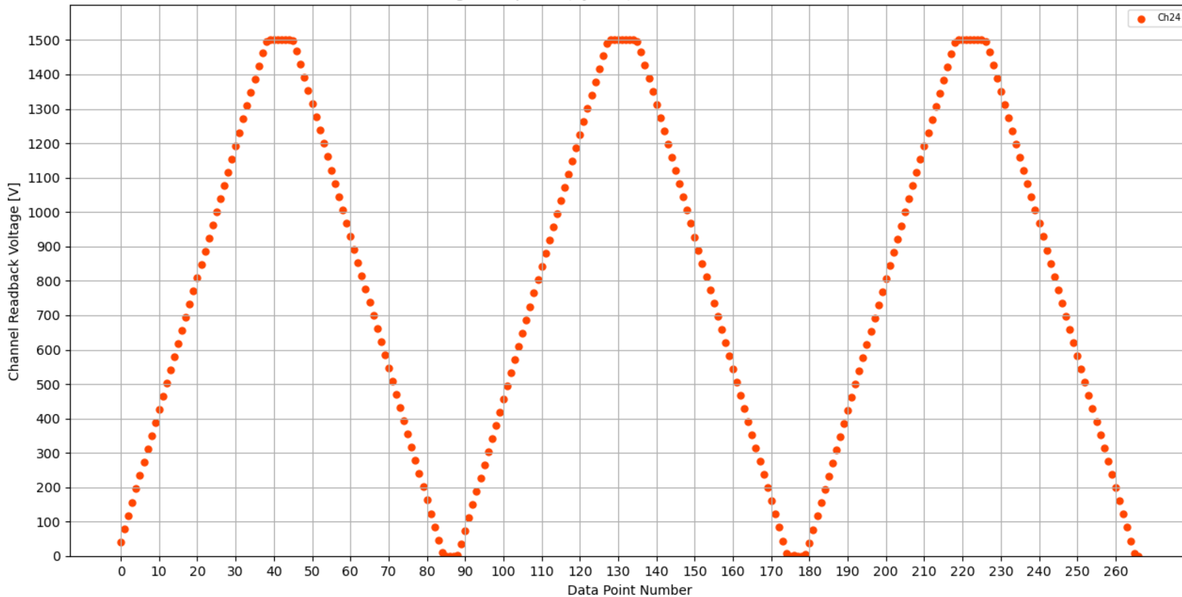
Voltage Ramp Test (Python) Bd #128, Slot #1, Ch #24
