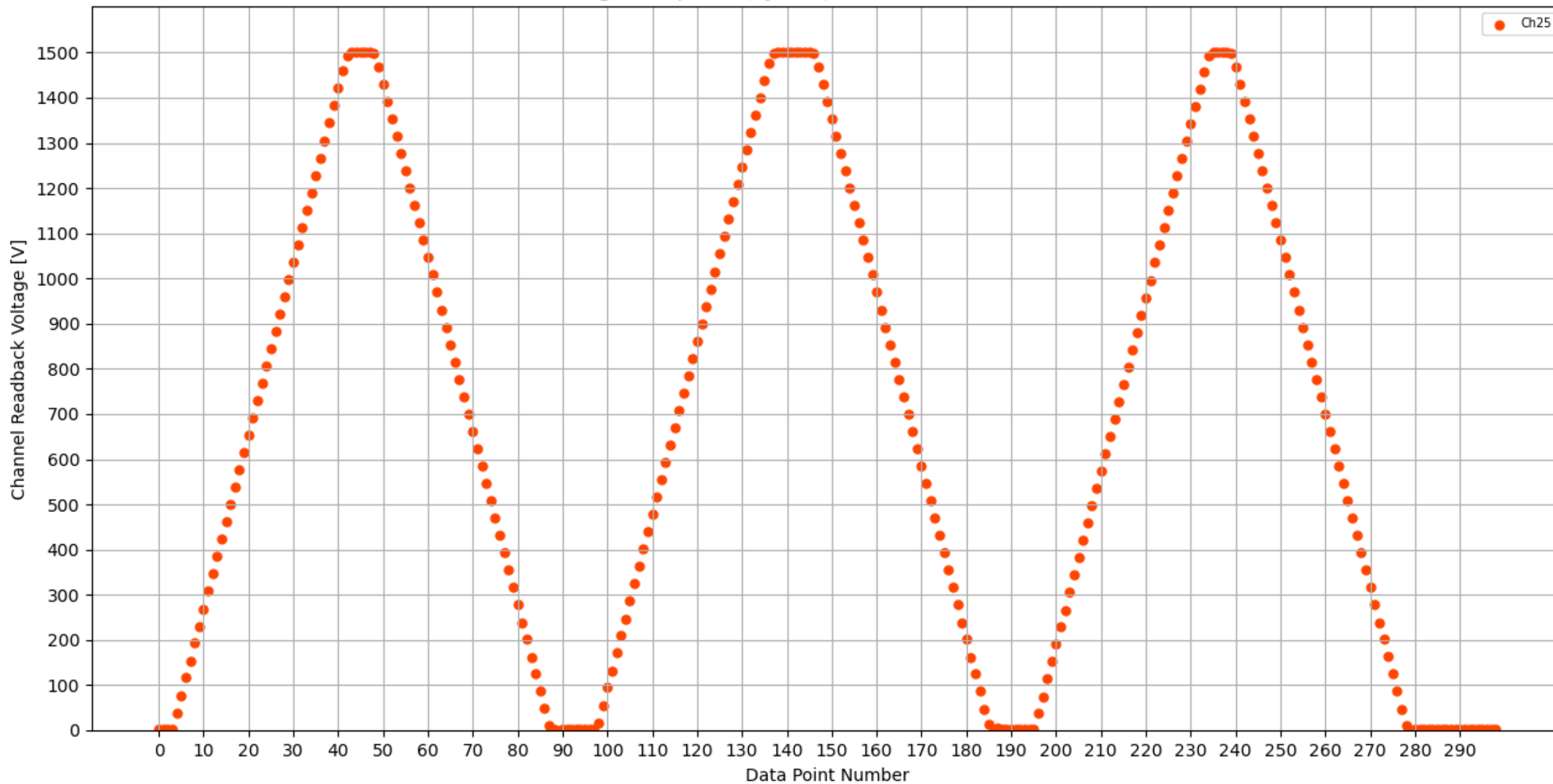
Voltage Ramp Test (Python) Bd #128, Slot #1, Ch #25
