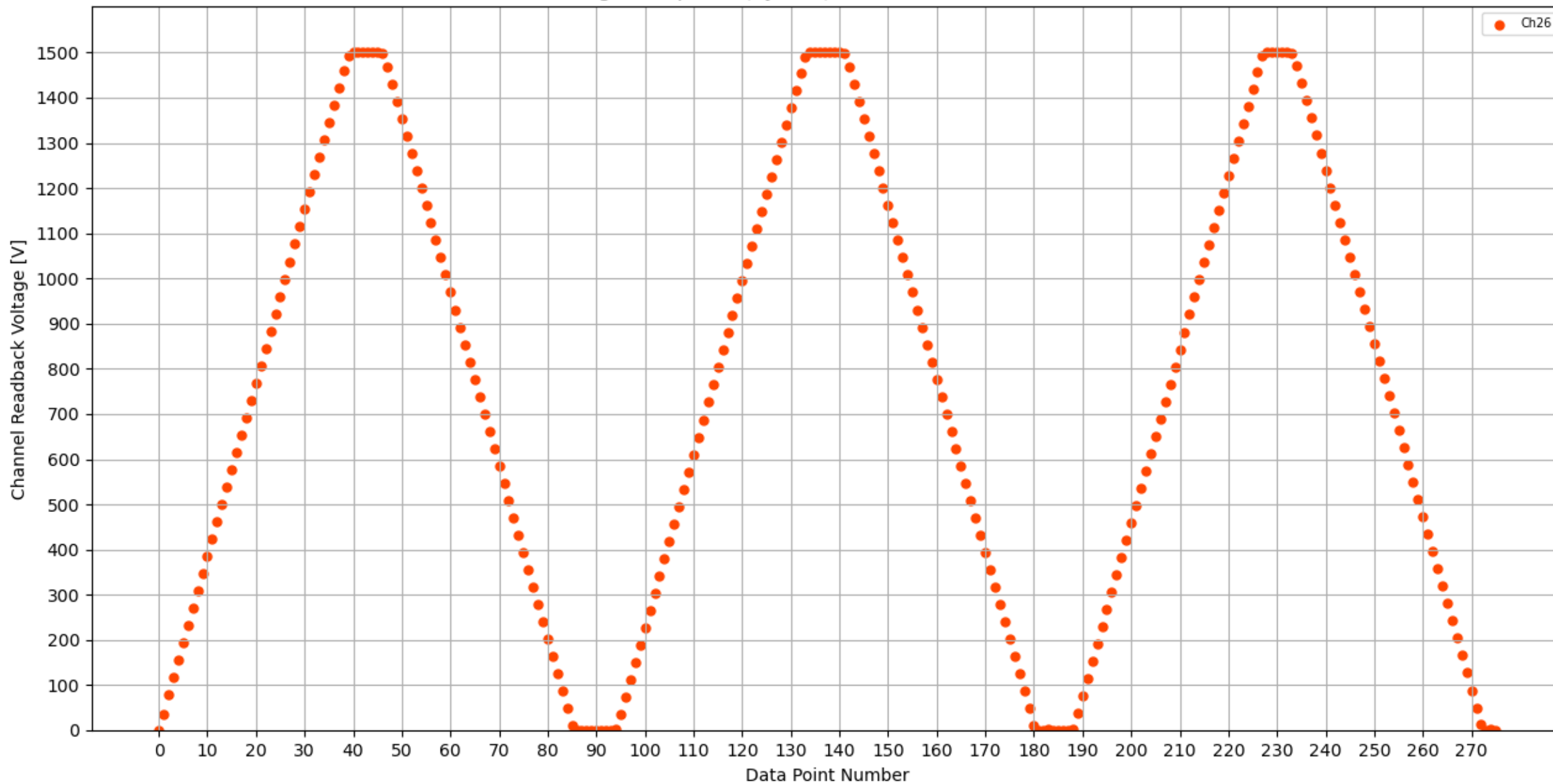
Voltage Ramp Test (Python) Bd #128, Slot #1, Ch #26
