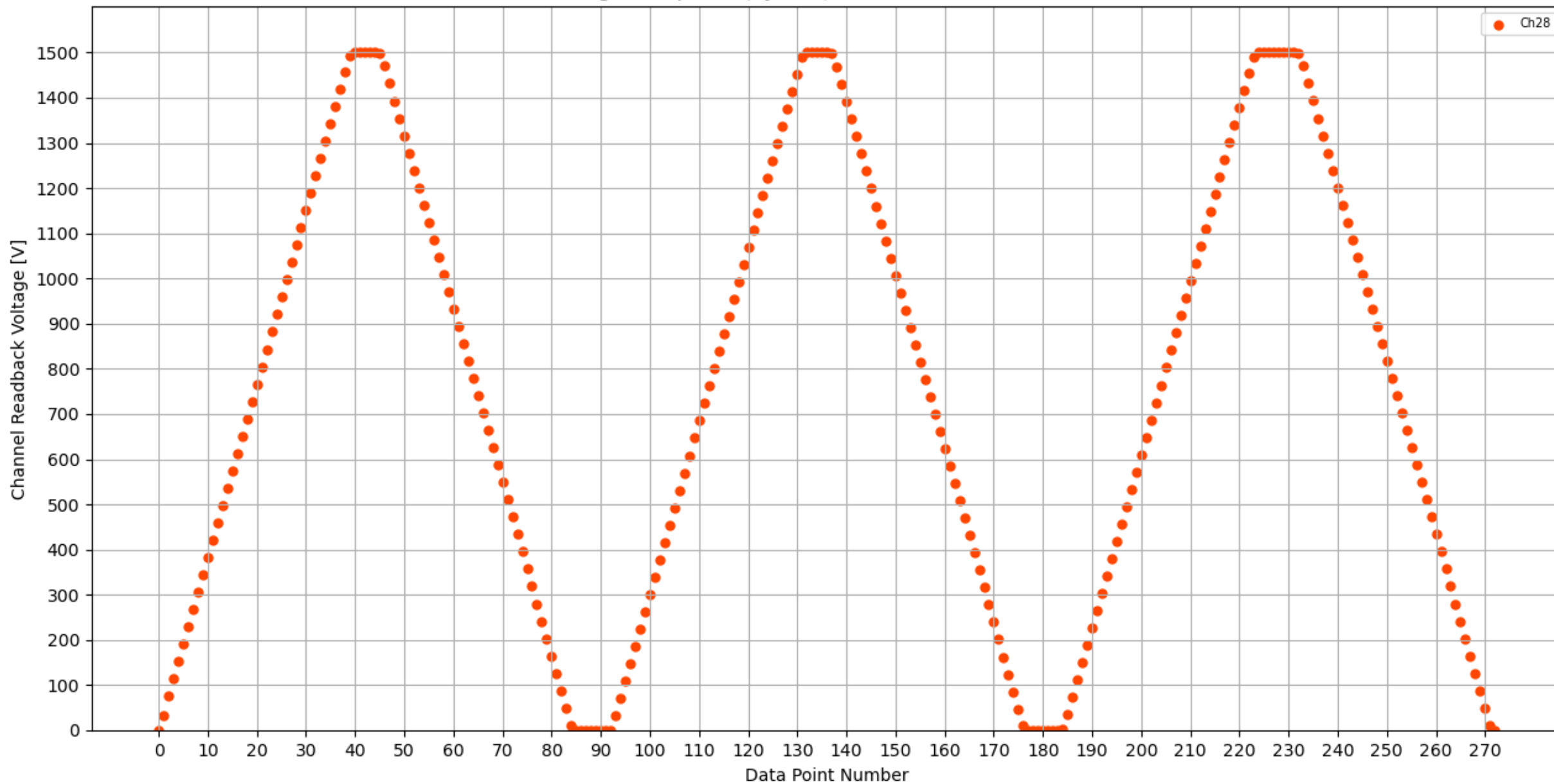
Voltage Ramp Test (Python) Bd #128, Slot #1, Ch #28
