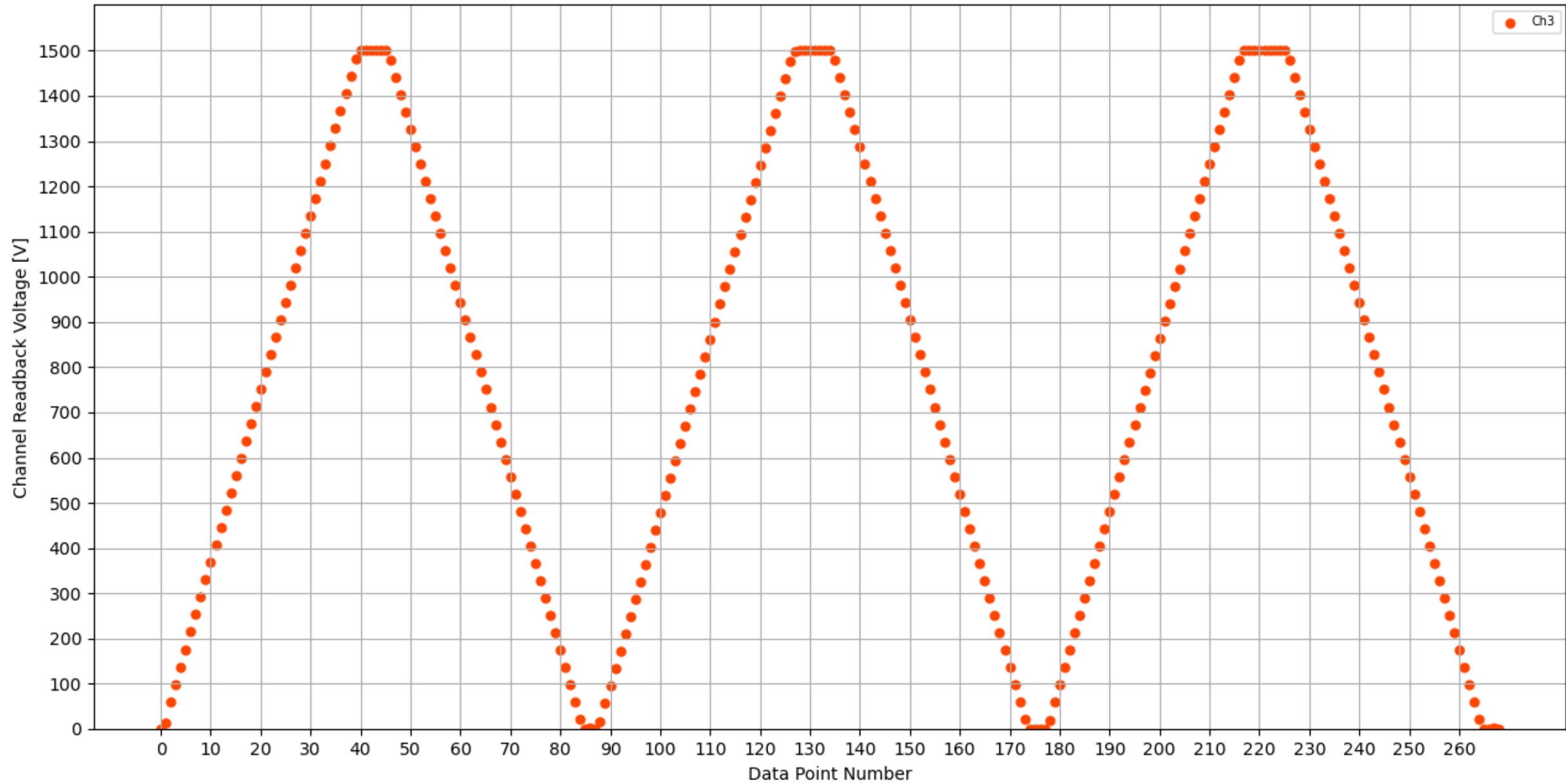
Voltage Ramp Test (Python) Bd #128, Slot #1, Ch #3
