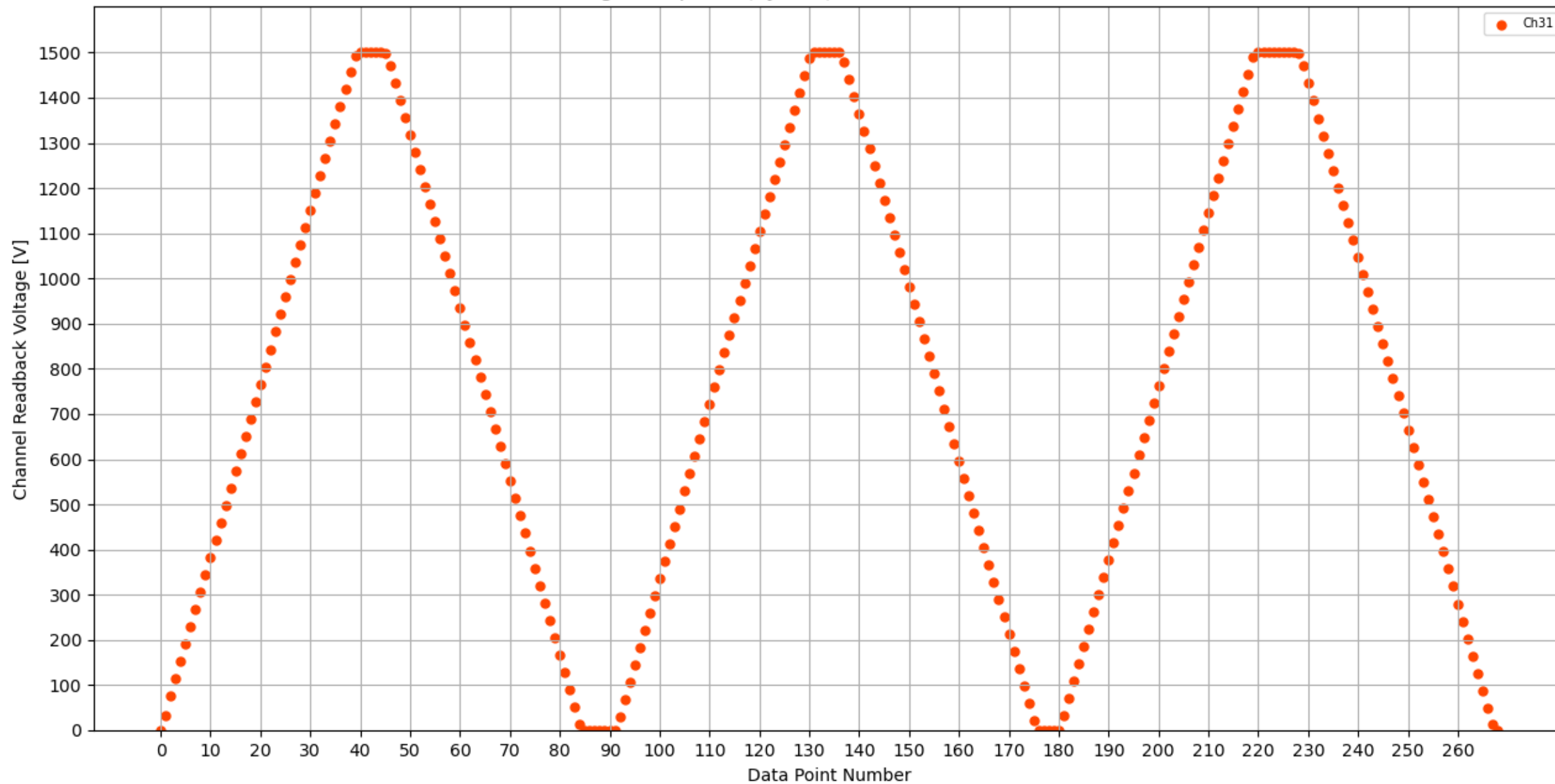
Voltage Ramp Test (Python) Bd #128, Slot #1, Ch #31
