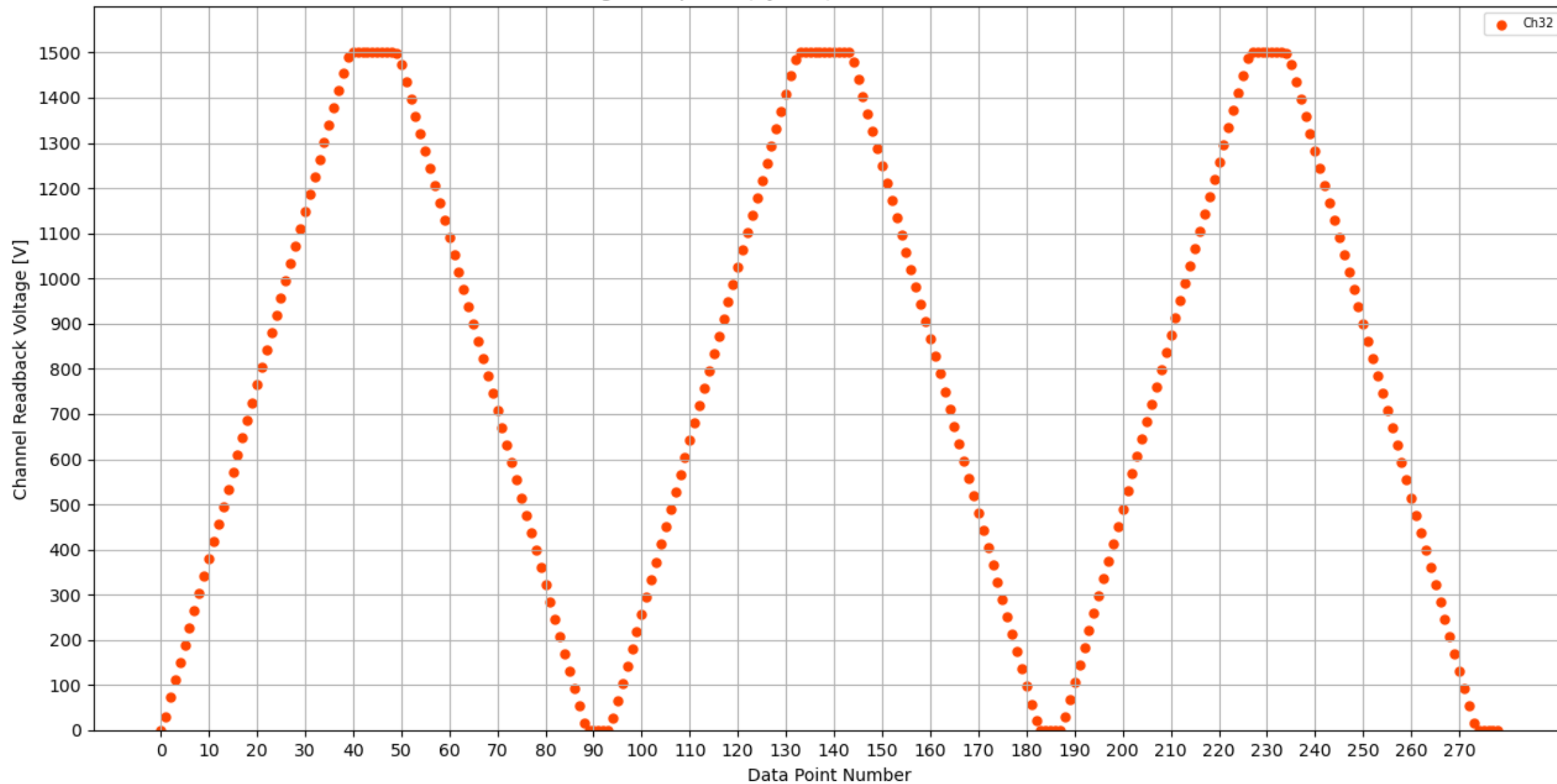
Voltage Ramp Test (Python) Bd #128, Slot #1, Ch #32
