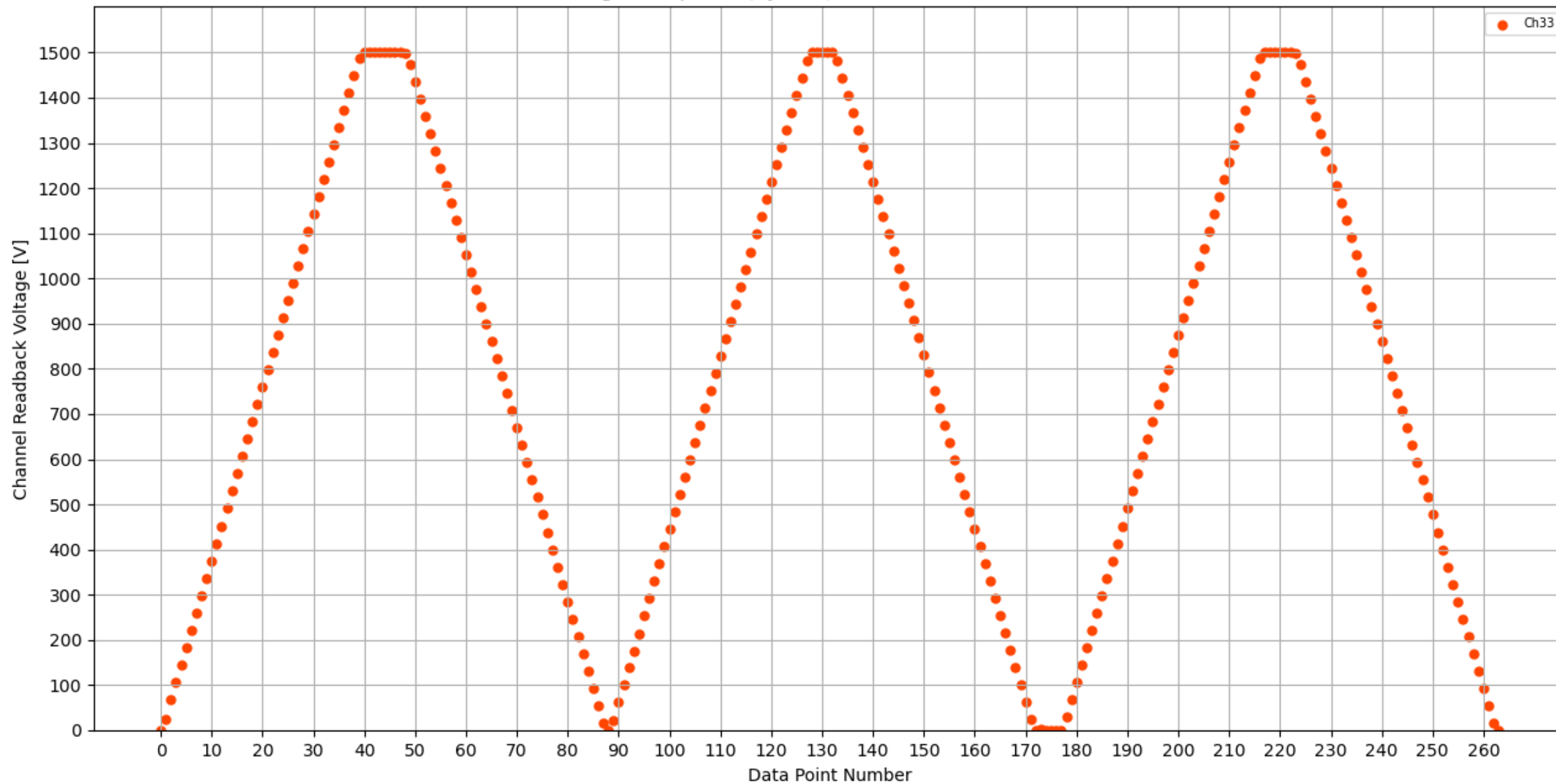
Voltage Ramp Test (Python) Bd #128, Slot #1, Ch #33
