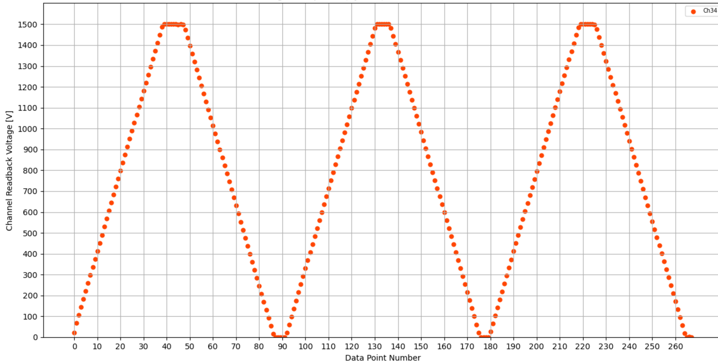
Voltage Ramp Test (Python) Bd #128, Slot #1, Ch #34
