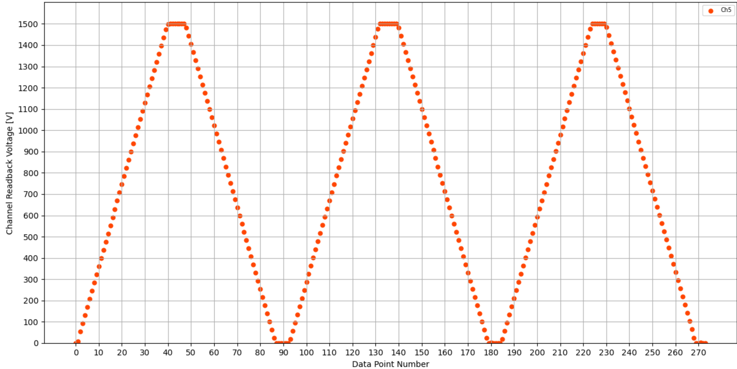
Voltage Ramp Test (Python) Bd #128, Slot #1, Ch #5
