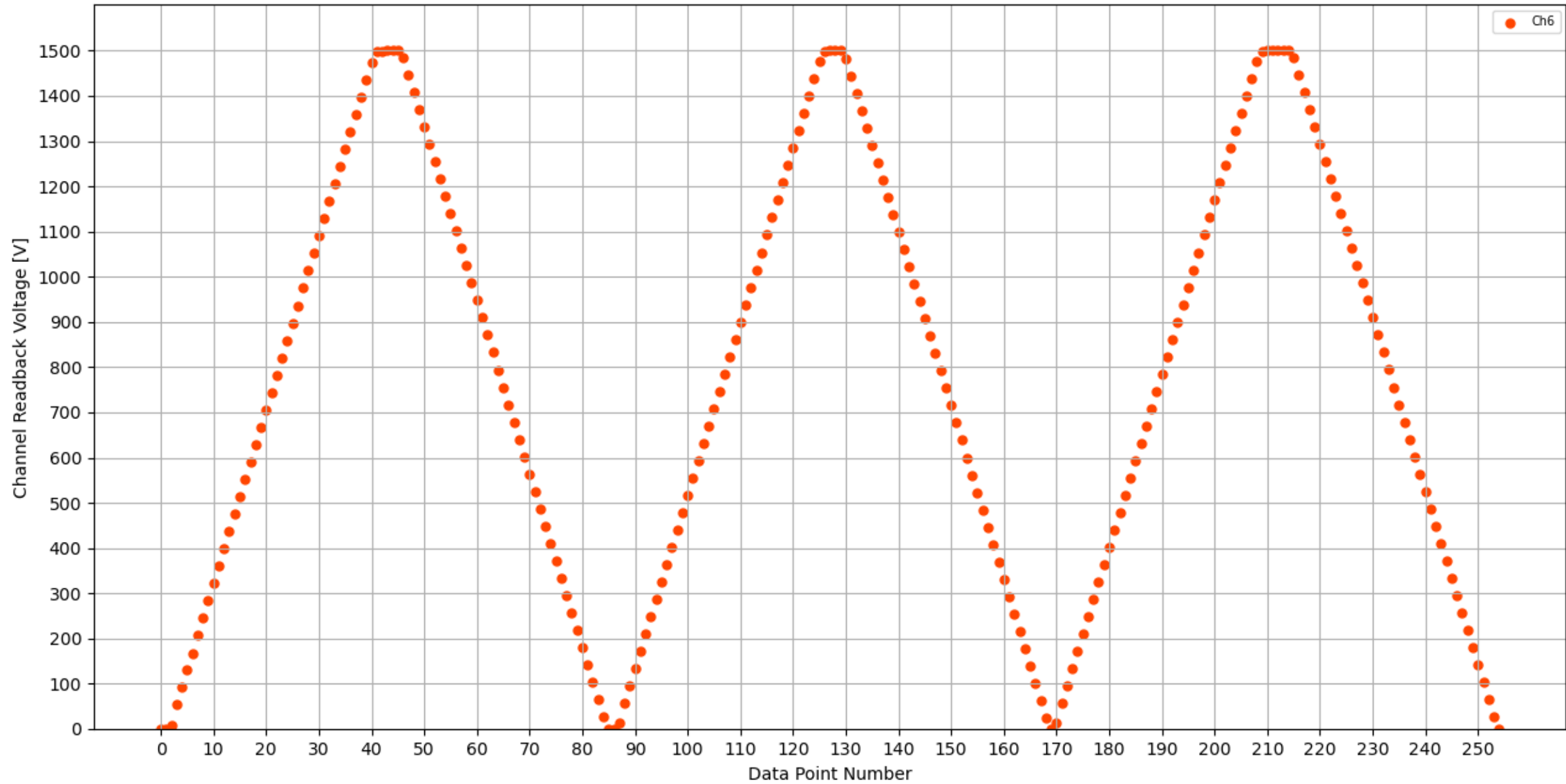
Voltage Ramp Test (Python) Bd #128, Slot #1, Ch #6
