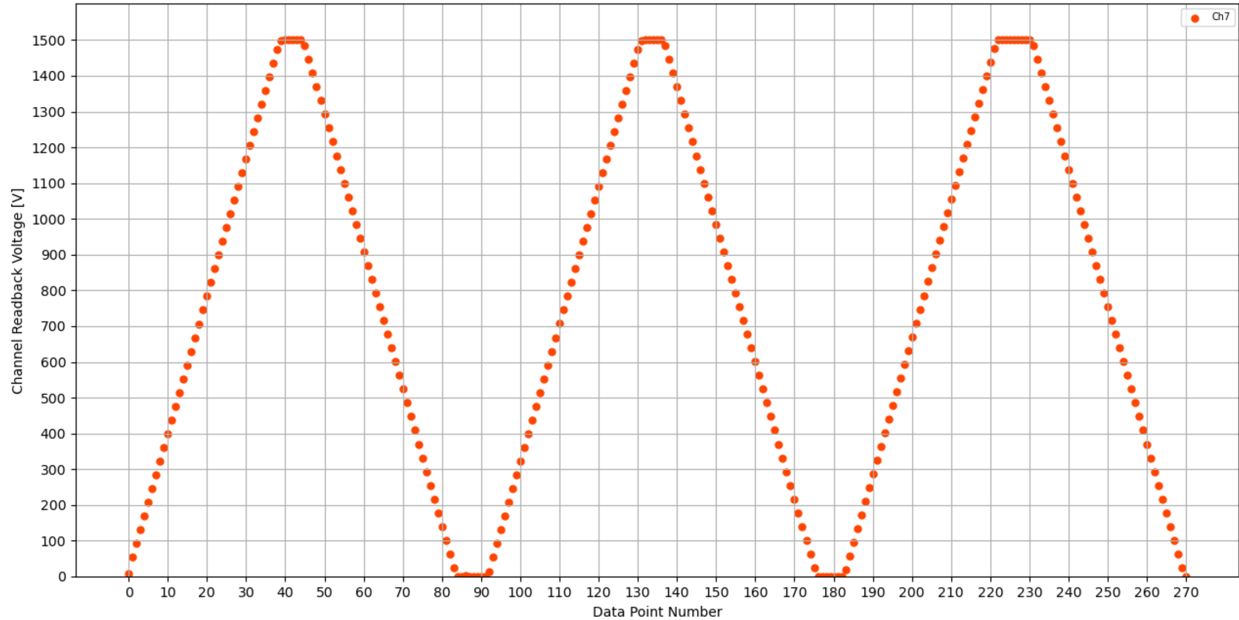
Voltage Ramp Test (Python) Bd #128, Slot #1, Ch #7
