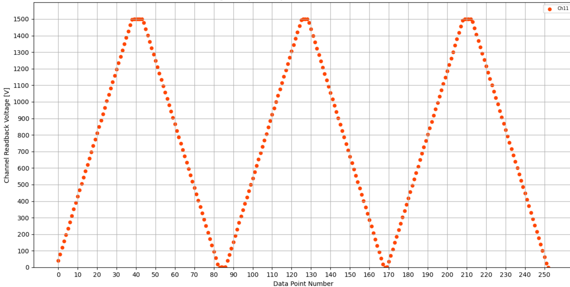
Voltage Ramp Test (Python) Bd #173, Slot #9, Ch #11
