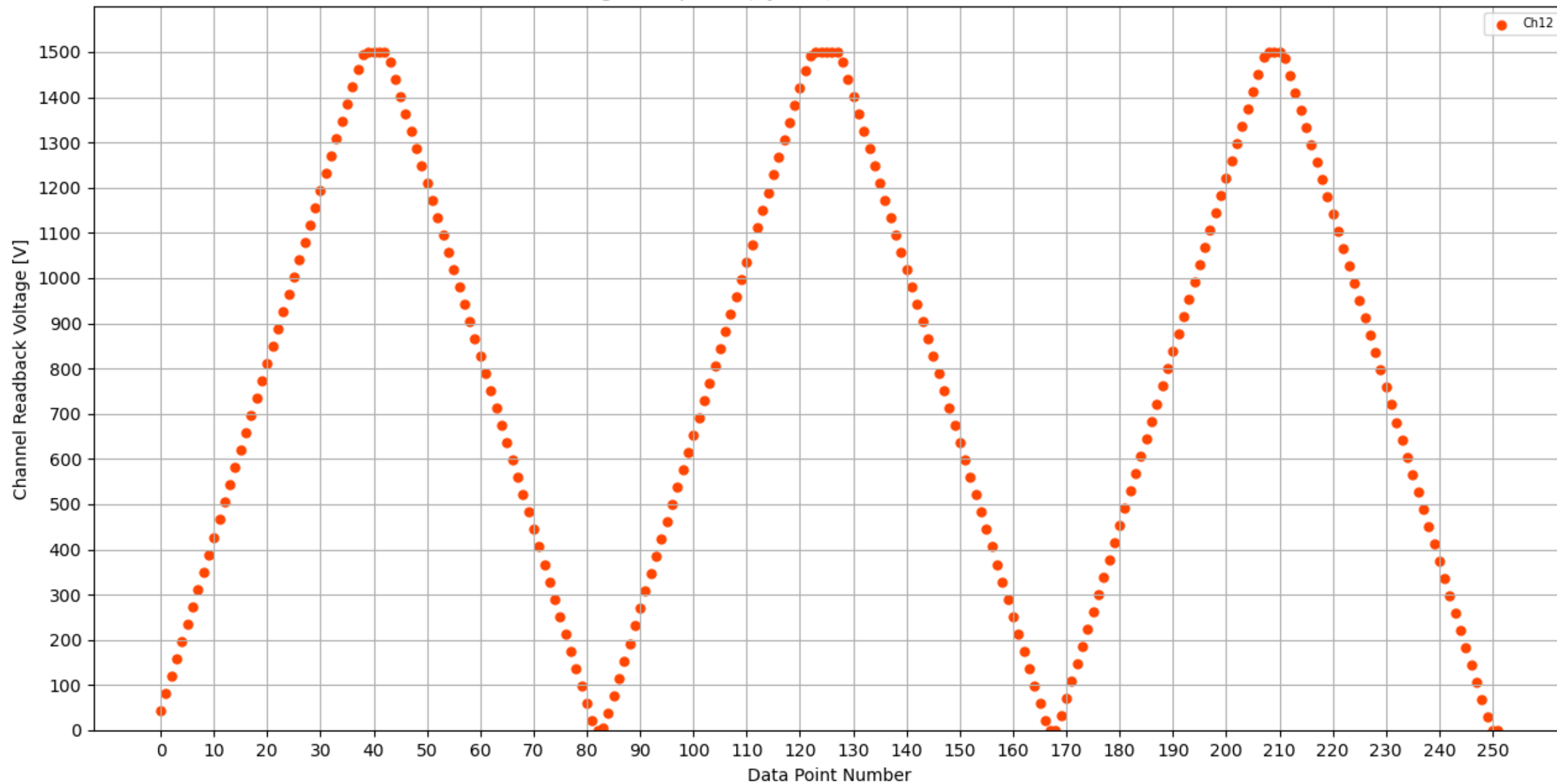
Voltage Ramp Test (Python) Bd #173, Slot #9, Ch #12
