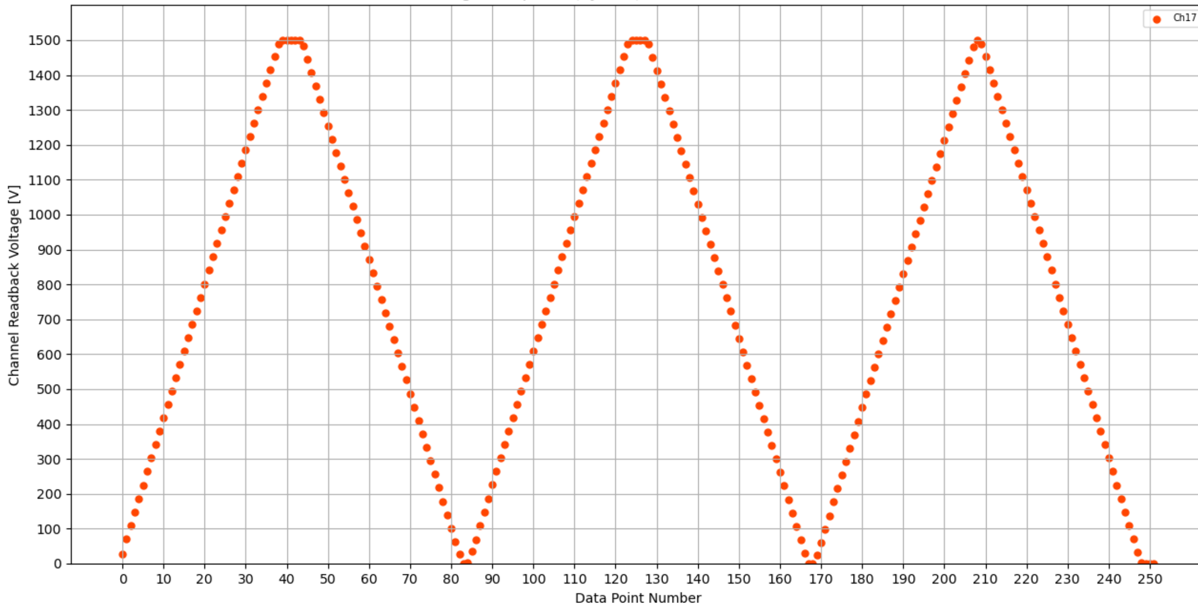
Voltage Ramp Test (Python) Bd #173, Slot #9, Ch #17
