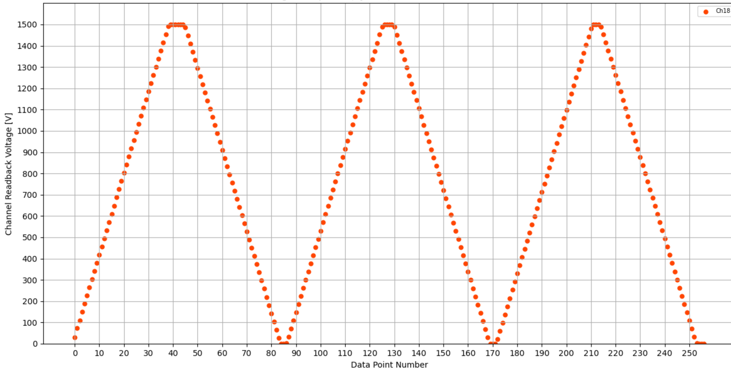
Voltage Ramp Test (Python) Bd #173, Slot #9, Ch #18
