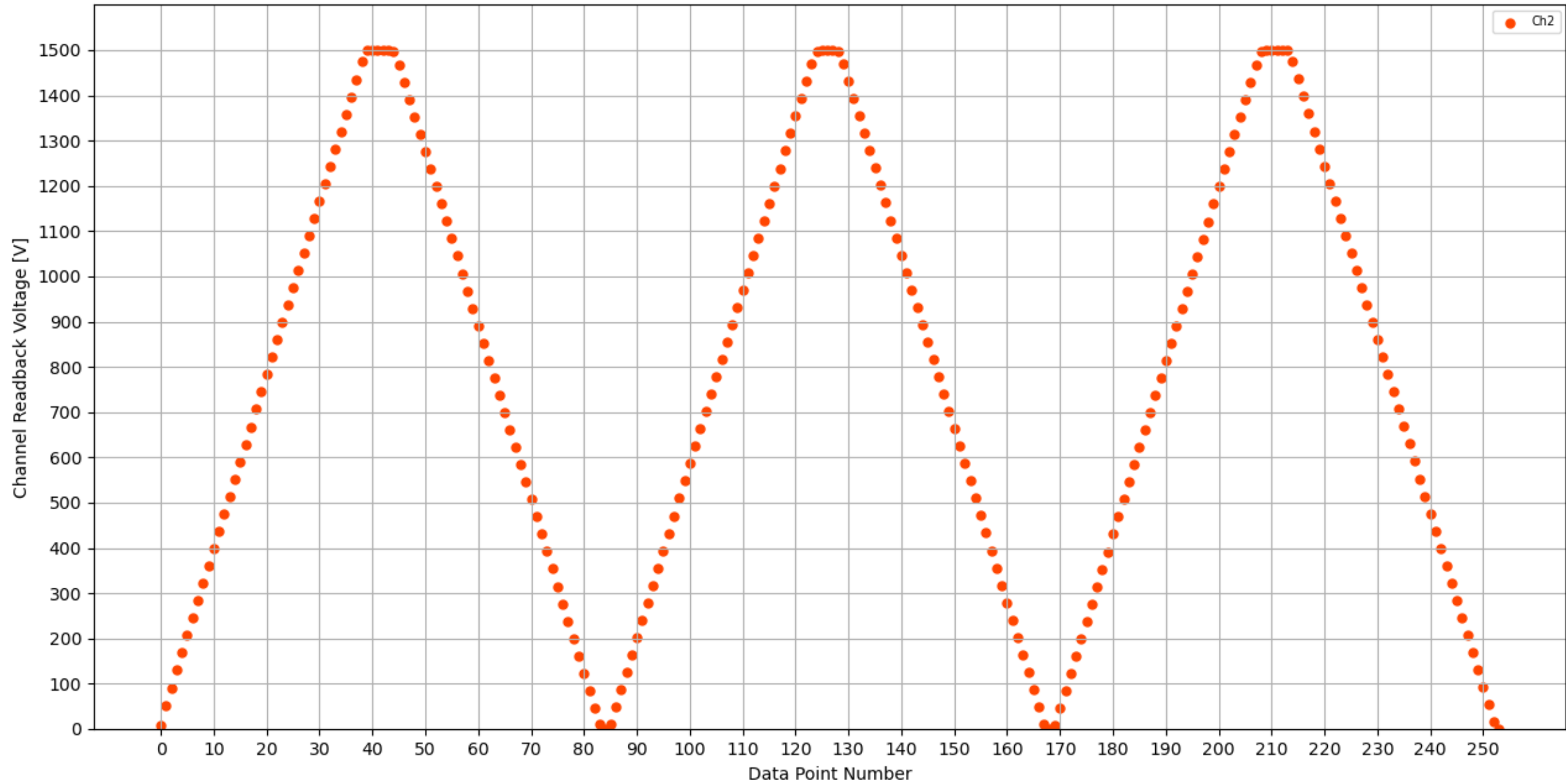
Voltage Ramp Test (Python) Bd #173, Slot #9, Ch #2
