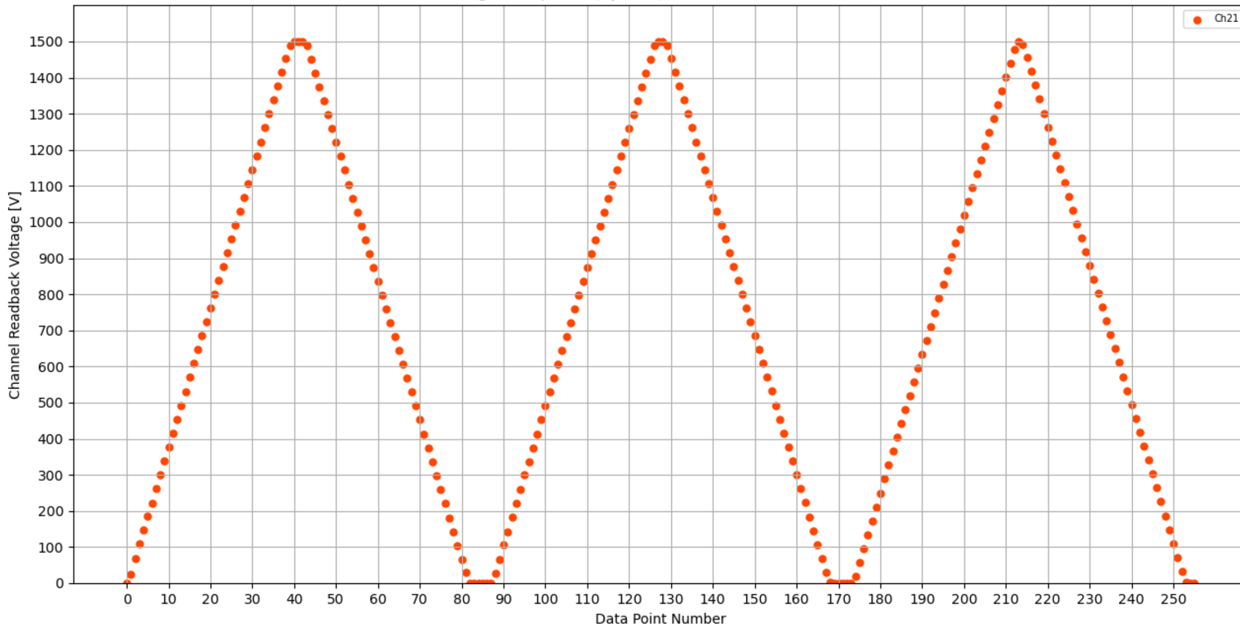
Voltage Ramp Test (Python) Bd #173, Slot #9, Ch #21
