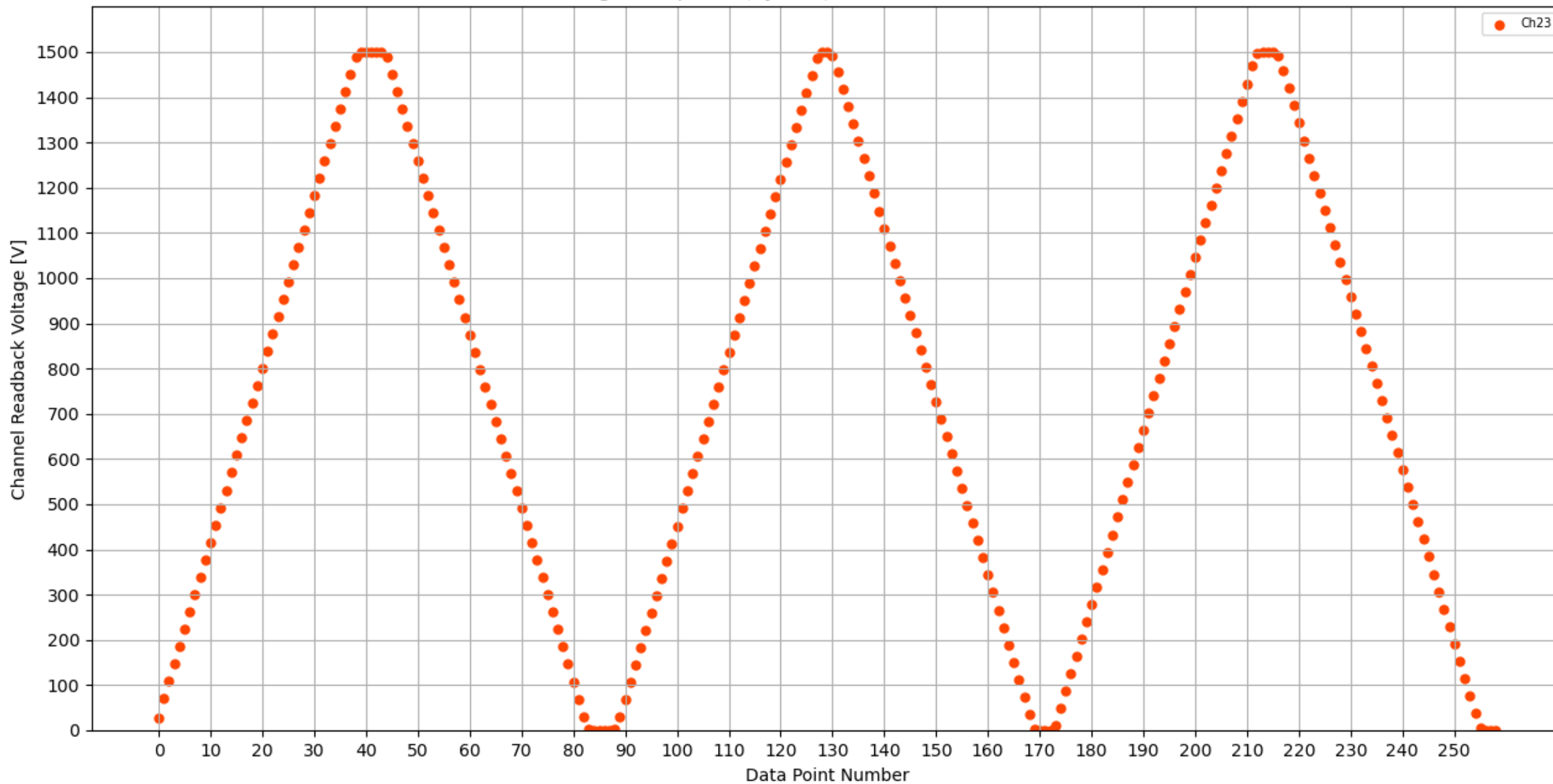
Voltage Ramp Test (Python) Bd #173, Slot #9, Ch #23
